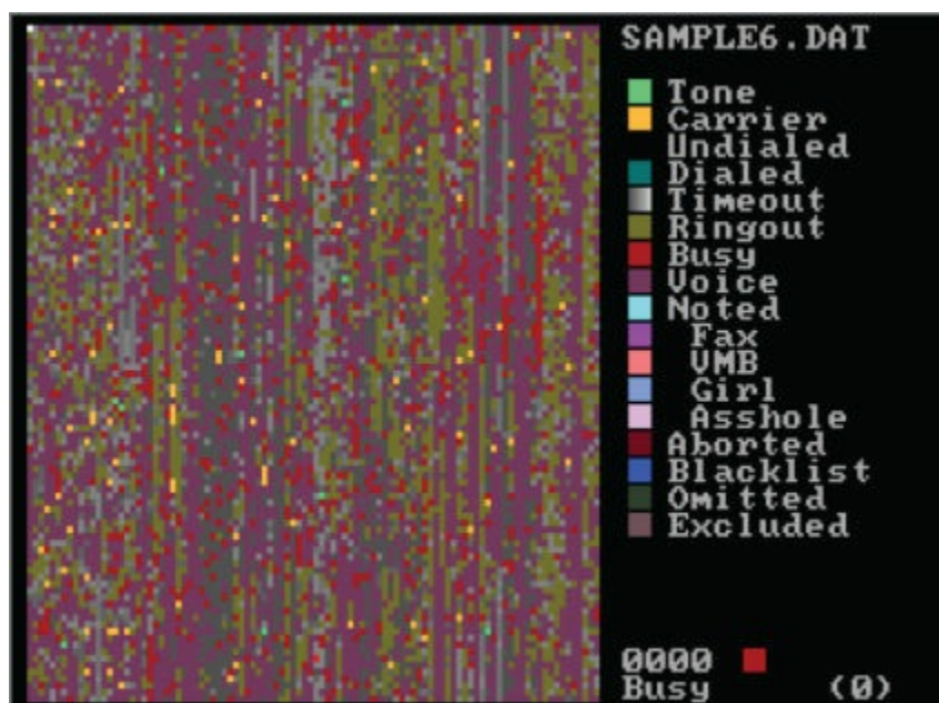
Figure 9.16: Toneloc output.
