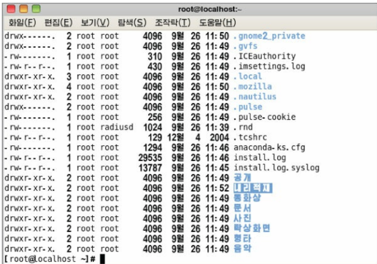
Figure 9.3: A shell.
