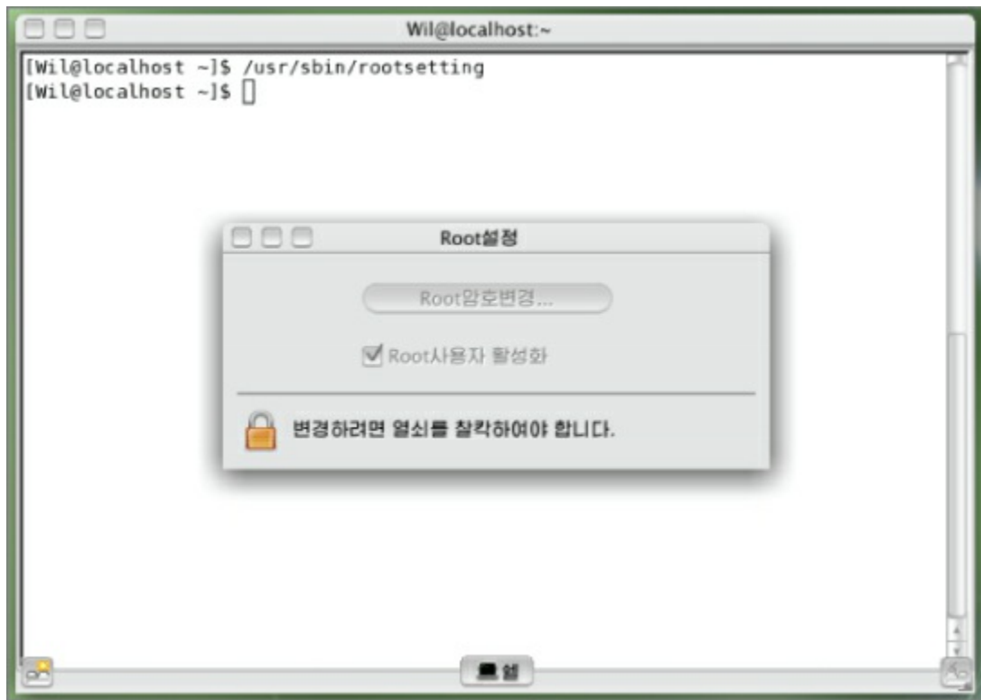
Figure 9.6: Run rootsetting.
