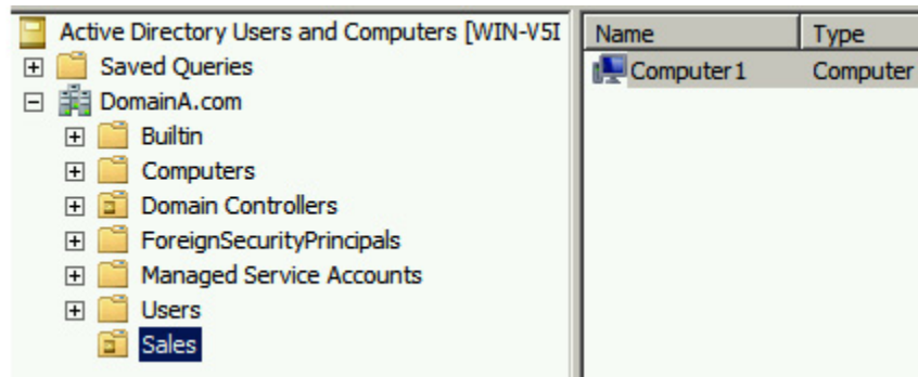
Figure 19.1: Active Directory
