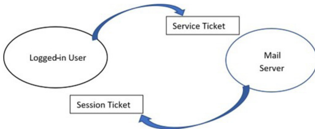
Figure 19.4: Mutual authentication
