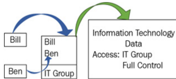
Figure 19.5: Group-based access
