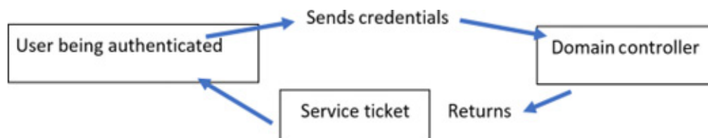
Figure 19.3: TGT
