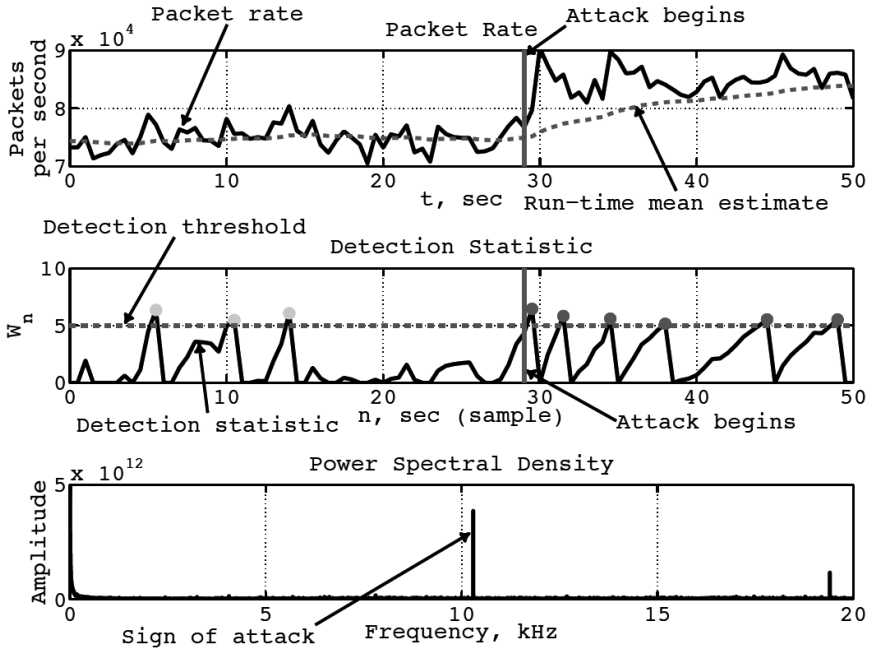
Fig. 2.14. Detection of the ICMP DDoS attack with HASIDS.
