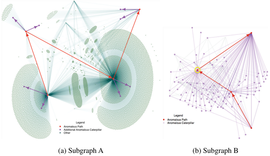
Fig. 3.5. Star, path, and caterpillar anomalies. Each subgraph has a core path, around which anomalous shapes were introduced. For each core path, the anomaly is plotted, along with the directly connected edges not involved in the anomaly, which are provided for context. Red edges and nodes give the core path, and additional caterpillar nodes and edges are plotted in purple. Every edge in subgraph B is part of the caterpillar for this subgraph. The yellow circle indicates the node at the center of the anomalous out-star.
