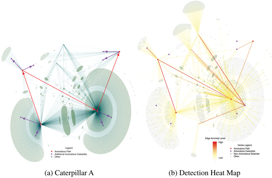
Fig. 3.7. Anomaly graph and heat map for Caterpillar A. The true anomaly is given on the left, with anomalous edges colored red and purple. Green nodes and edges are uninvolved in the anomaly, but are provided to give context. The more green edges, the more chance of false discovery. The detected heat map is displayed on the right, with darker red indicating more evidence of an anomaly.
