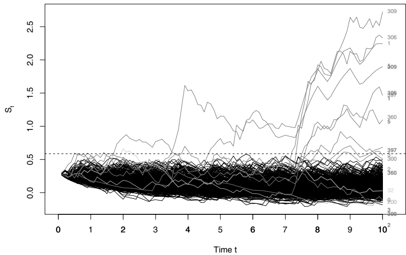
Fig. 6.13. VAST data control charts: continuous time model for incoming event times for each node.
