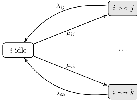
Fig. 6.5. Generalised undirected Markov model. i \leftrightarrow j denotes i and j connecting in either direction.
