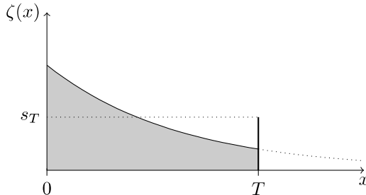
Fig. 6.10. Example of a time to event variable X of mixed type, due to right-censoring at T .
