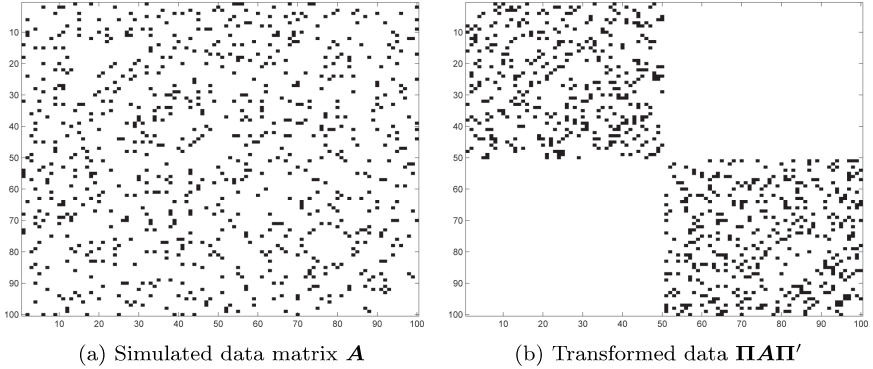
Fig. 1.3. Representations \mathbf{A} and \mathbf{\Pi A \Pi'} of data drawn from the stochastic block model of Example 1.3, corresponding to isomorphic graphs (black boxes denote links). Though p_{01} = 0 , only a small subset of permutation similarity transformations \mathbf{\Pi}(\cdot)\mathbf{\Pi'} will reveal the disconnected nature of this network.
