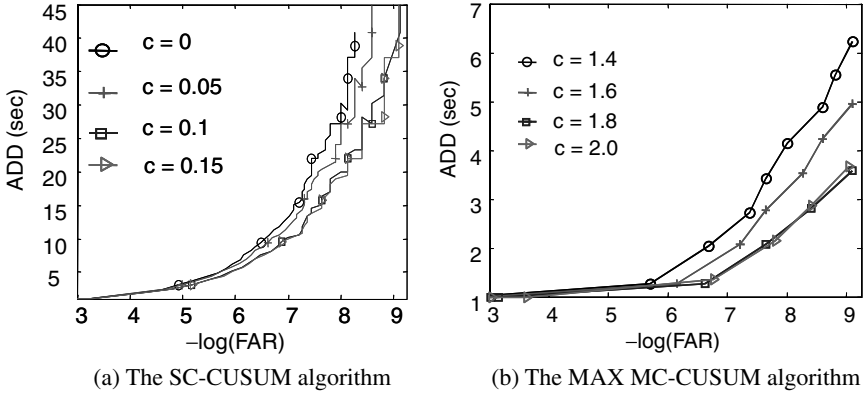
Fig. 2.5. ADD versus -\log(\text{FAR}) for the SC-CUSUM and MAX MC-CUSUM algorithms.
