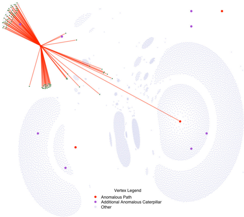
Fig. 3.8. Star scanning results for Caterpillar A. Detected edges are plotted in red. The light blue nodes are to provide context.
