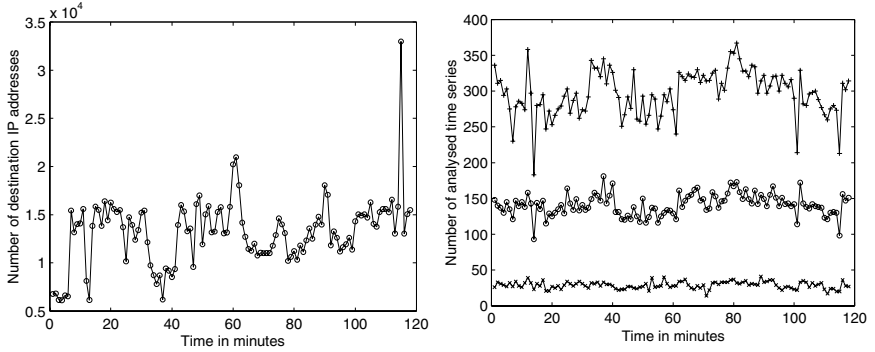
Fig. 5.2. Left: Number of destination IP addresses every minute. Right: Number of analysed time series every minute when M' = 1 (“x”), M' = 5 (“o”) and M' = M = 10 (“+”).
