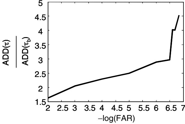
Fig. 2.11. Relative efficiency versus -\log \text{FAR} .
