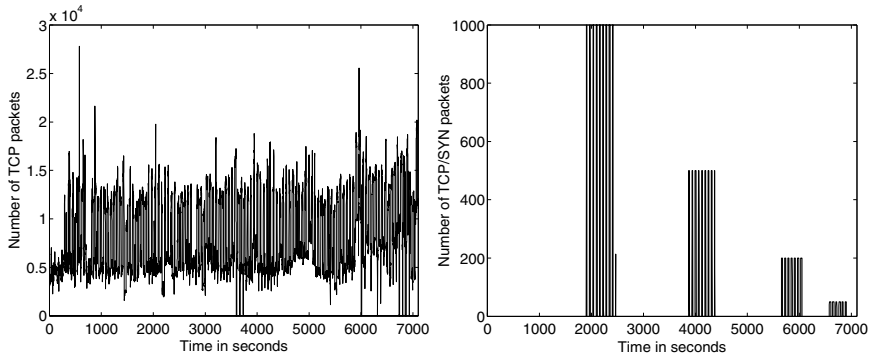
Fig. 5.1. Number of TCP packets exchanged and number of TCP/SYN packets received by the four attacked IP addresses.
