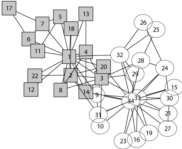
Fig. 1.4. Visualization of the Zachary karate data of Section 1.4.1. Nodes are numbered and binary categorical covariate values, reflecting the subsequent group split, are indicated by shape.
