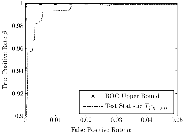
Fig. 1.6. ROC curve of T_{\widehat{LR-FD}} using fixed-degree models for both the null and alternate hypotheses. (The stepped appearance of the curve is an artifact of the importance sampling weights.) Also shown is an ROC upper bound, obtained using knowledge of the true group membership for each node.
