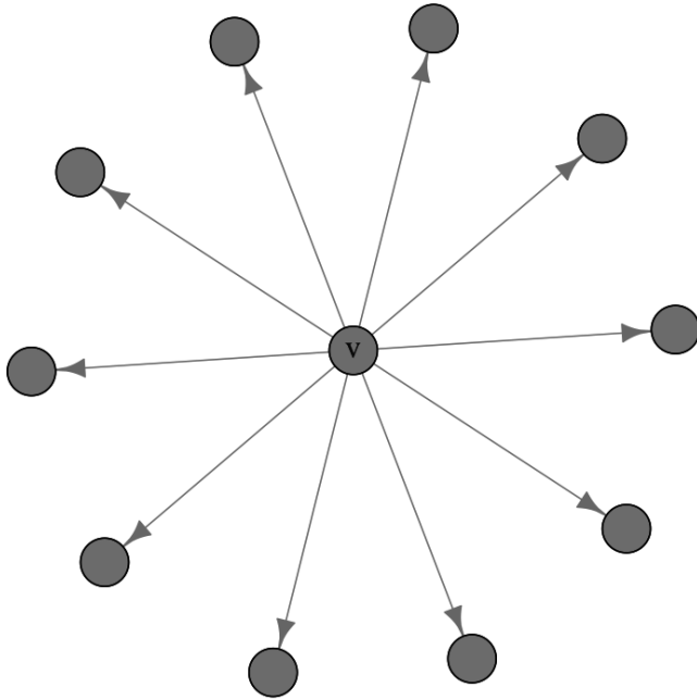
Fig. 3.3. Example out-star, centered at node v .
