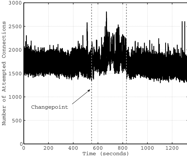
Fig. 2.6. The connections birth rate for LANDER data.
