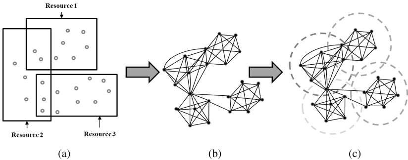
Fig. 4.2. Steps of topic extraction: (a) resource-tag graph (GRL); (b) tag concept hierarchy; and (c) topic extraction (TC).
