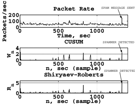
Fig. 2.12. Spam detection. Top – raw data; middle – CUSUM statistic; bottom – SR statistic.
