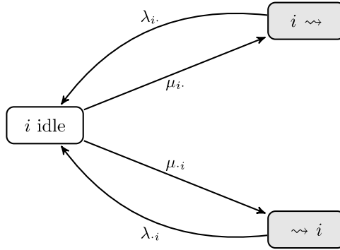
Fig. 6.4. Three-state “idle-connected” directed Markov model. i \rightsquigarrow denotes i initiating a connection, whilst \rightsquigarrow i denotes i receiving a connection.
