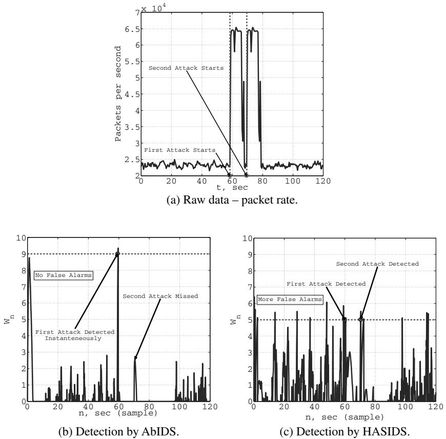
Fig. 2.15. Detection of a short UDP DoS attack with AbIDS and HASIDS. The second “pulse” is missed by the AbIDS but not by the HASIDS.
