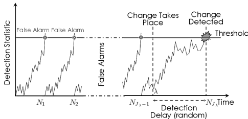
Fig. 2.2. Illustration of the typical multi-cyclic surveillance scenario.
