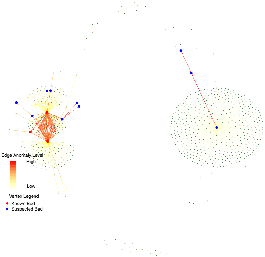
Fig. 3.10. Real detection heat map. Red nodes were independently verified as being compromised during the attack. Blue nodes were highly suspicious (low p -values on edges associated with these nodes).
