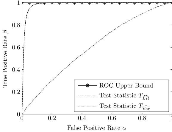
Fig. 1.5. Receiver operating characteristic (ROC) curves corresponding to tests of the data of Section 1.4.1, with Erdős–Rényi null and two-group stochastic block model alternate. Test statistics T_{\widehat{LR}} and T_{\widehat{Var}} were calculated via simulation, with the ROC upper bound obtained using knowledge of the true group membership for each node.
