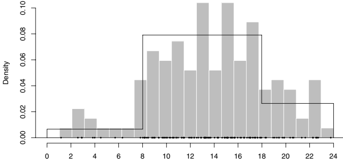
Fig. 6.8. Estimated m_3(s) using the VAST data for individual 3, compared with a histogram of those data.
