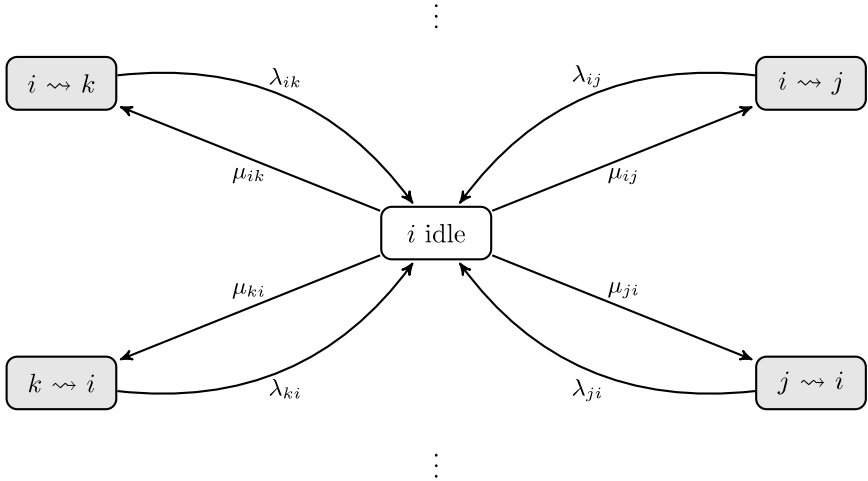
Fig. 6.6. Generalised directed Markov model. i \rightsquigarrow j denotes i initiating a connection with node j .
