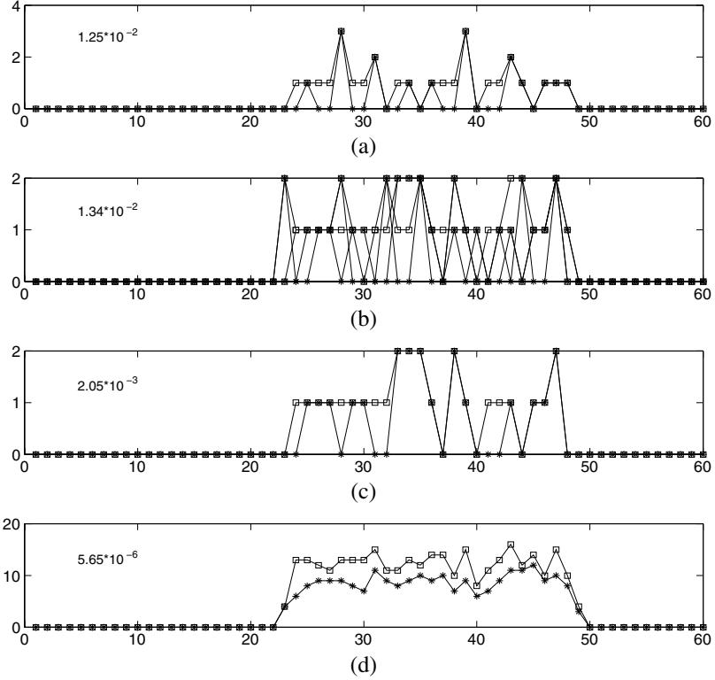
Fig. 5.6. (a), (b), (c): times series (\underline{X}_i^{(k)}(t), t = 1, \dots, 60) and (\overline{X}_i^{(k)}(t), t = 1, \dots, 60) displayed with (*) and (□), respectively, for three different values of k , (d): (\underline{Z}_i(t), t = 1, \dots, 60) and (\overline{Z}_i(t), t = 1, \dots, 60) displayed with (*) and (□), respectively.
