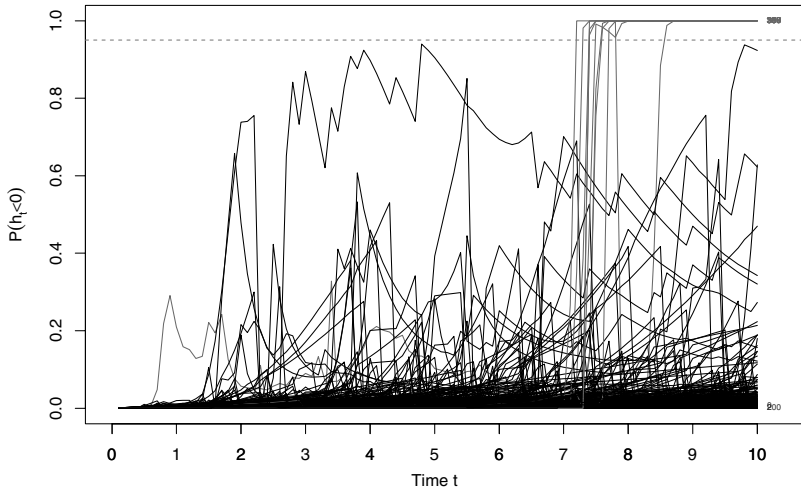
Fig. 6.18. VAST data \mathbb{P}(h(t) < 0) : continuous time model for incoming event times for each node.
