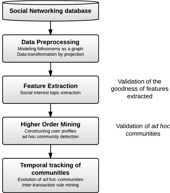
Fig. 4.1. The three-step framework consists of data preprocessing, feature extraction, and higher-order mining.
