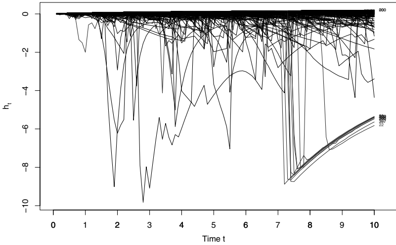
Fig. 6.17. VAST data \mathbb{E}[h(t)] : continuous time model for incoming event times for each node.
