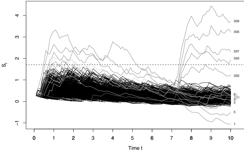
Fig. 6.16. VAST data control charts: continuous time models for incoming and outgoing event times for each edge of a node.
