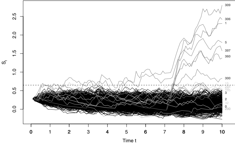
Fig. 6.11. VAST data control charts: continuous time model for undirected node event times.
