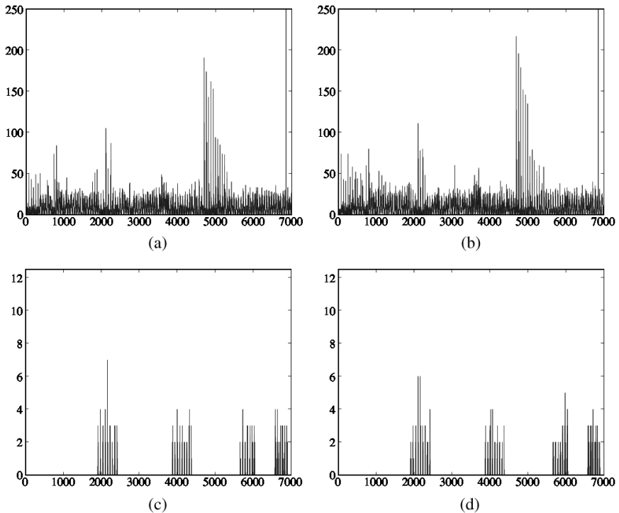
Fig. 5.5. Number of TCP/SYN packets globally exchanged within two particular monitors (a), (b) and received by the four attacked IP addresses within these two particular monitors (c), (d). (a) and (c) correspond to the traffic in monitor 1. (b) and (d) correspond to the traffic in monitor 2.
