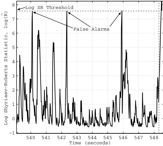
Fig. 2.7. Long run of the SR procedure (logarithm of the SR statistic versus time) for SYN flood attack.
