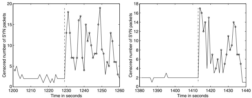
Fig. 5.4. Censored time series for IP addresses considered as false alarms where the vertical lines correspond to the detected changepoint instants and the uncensored values are displayed with (“o”).
