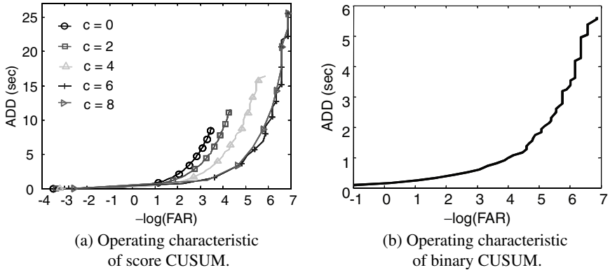
Fig. 2.10. SADD (sec) versus -\log \text{FAR} for the score-based and binary CUSUM algorithms.
