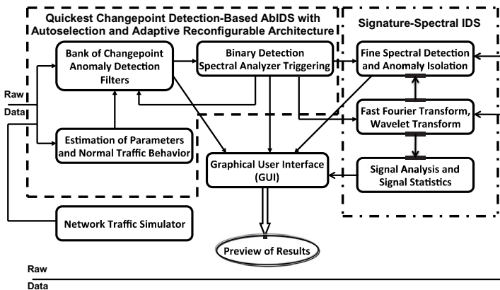
Fig. 2.13. Block diagram of the hybrid anomaly–signature intrusion detection system.
