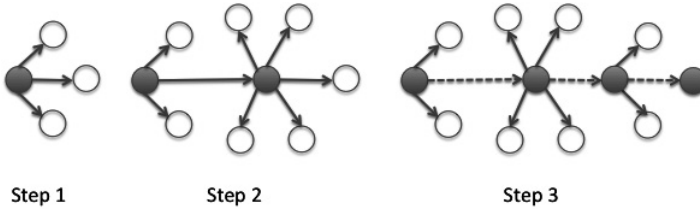
Fig. 3.2. A traversal attack. Step 1: Initial infection and local search. Step 2: First traversal has occurred, and further search is performed. Step 3: A full traversal has occurred. This shape is denoted as a caterpillar . The data on each edge in this graph is potentially anomalous. The filled nodes and dotted edges in Step 3 form a 3-path, which is one type of shape used to capture this behavior.
