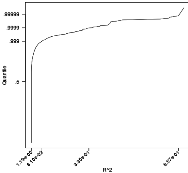
Fig. 3.4. Empirical CDF of absolute value of correlations between pairs of edges connected in a 2-path.
