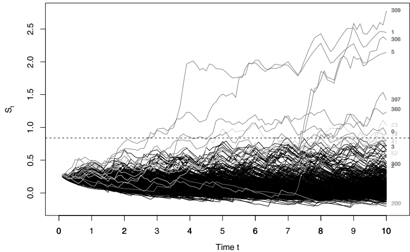
Fig. 6.14. VAST data control charts: continuous time model for incoming event times and Markov model for corresponding incoming caller for each node.
