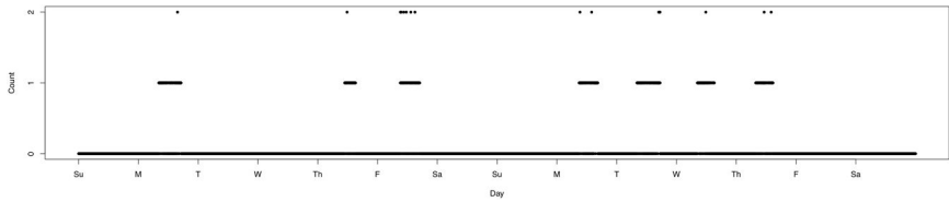
Fig. 3.1. Counts of connections per minute between two machines in LANL's internal network. The connections originate at a specific user's machine, and the destination is a server providing virtual desktop services.
