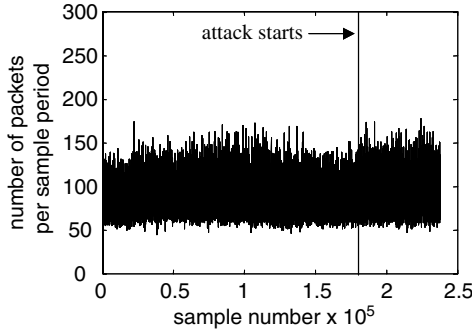
Fig. 2.9. Time series of the total number of UDP packets in a sample period 0.015 msec. Observe that the attack is not visible to the naked eye.
