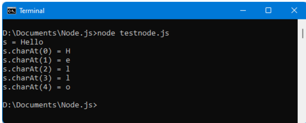
Figure 2.27 – Using the charAt() method
