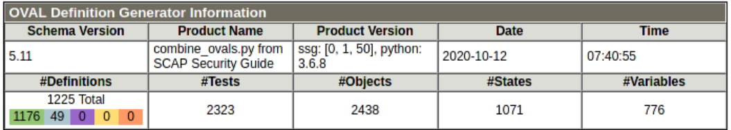
Figure 11.3 – OpenSCAP test scan definitions summary
