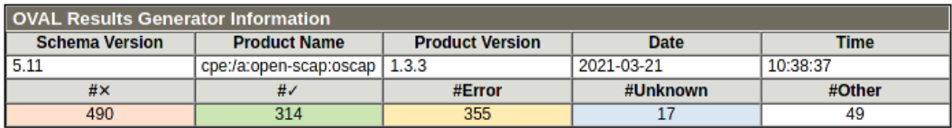
Figure 11.2 – OpenSCAP test scan summary
