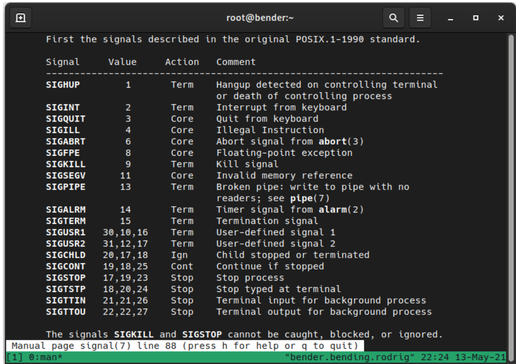
Figure 16.2 – Listing of signals, number equivalent, disposition (action), and behavior (man 7 signal)
