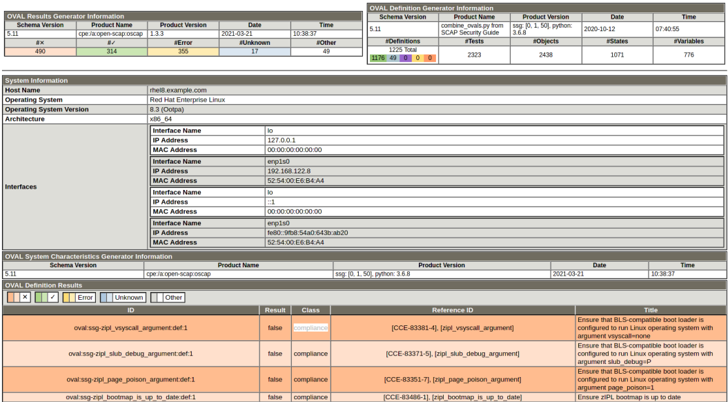
Figure 11.1 – Initial results of an OpenSCAP test scan
