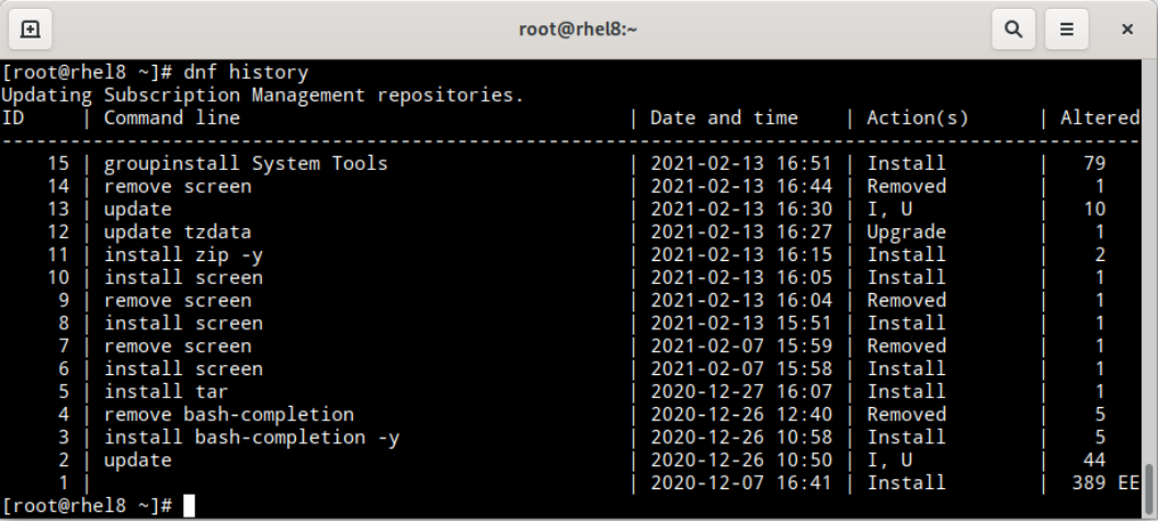
Figure 7.15 – Partial capture of RHEL dnf/yum history
