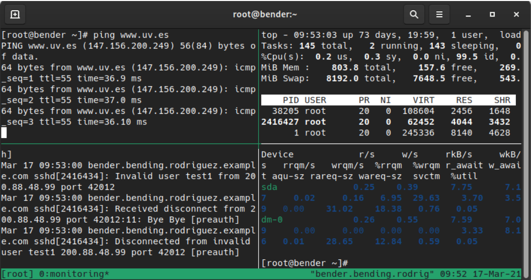
Figure 8.21 – tmux with four panes running different commands inside the same window
