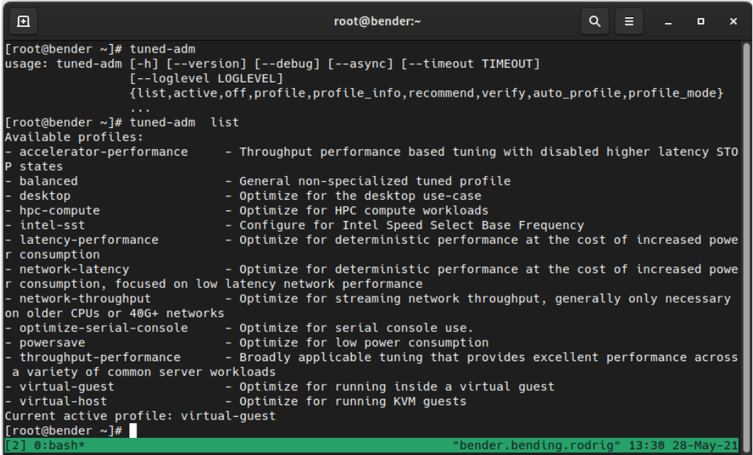
Figure 16.5 – The tuned-adm command-line options and profiles
