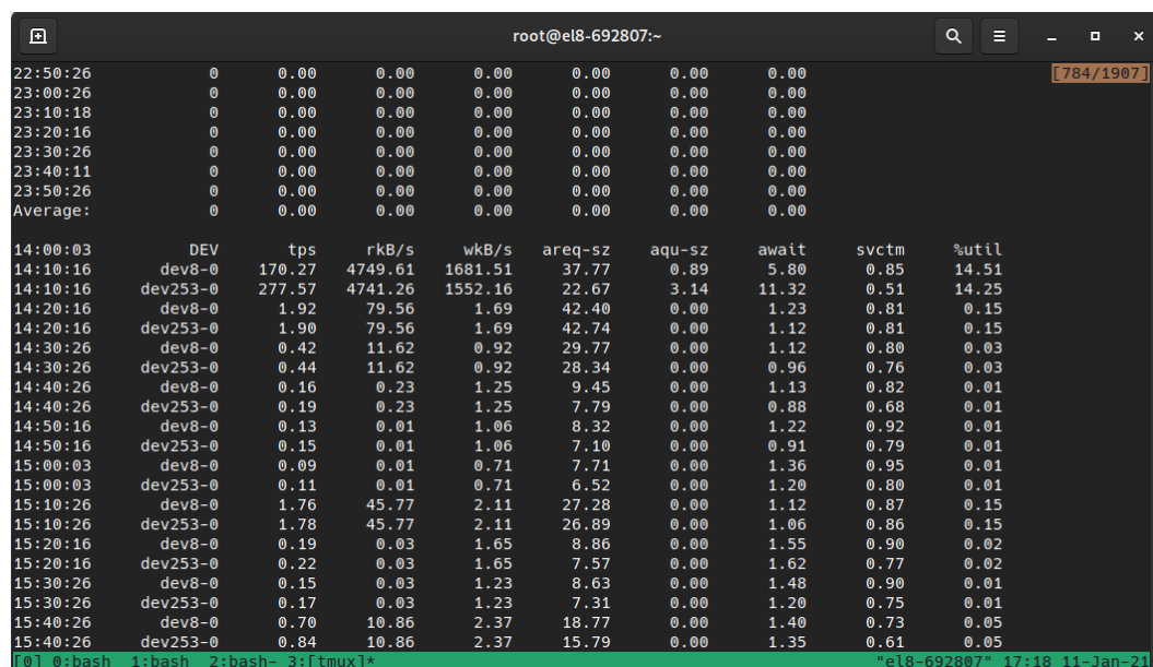
Figure 4.9 – Contents of /var/log/sar02 on the example system
