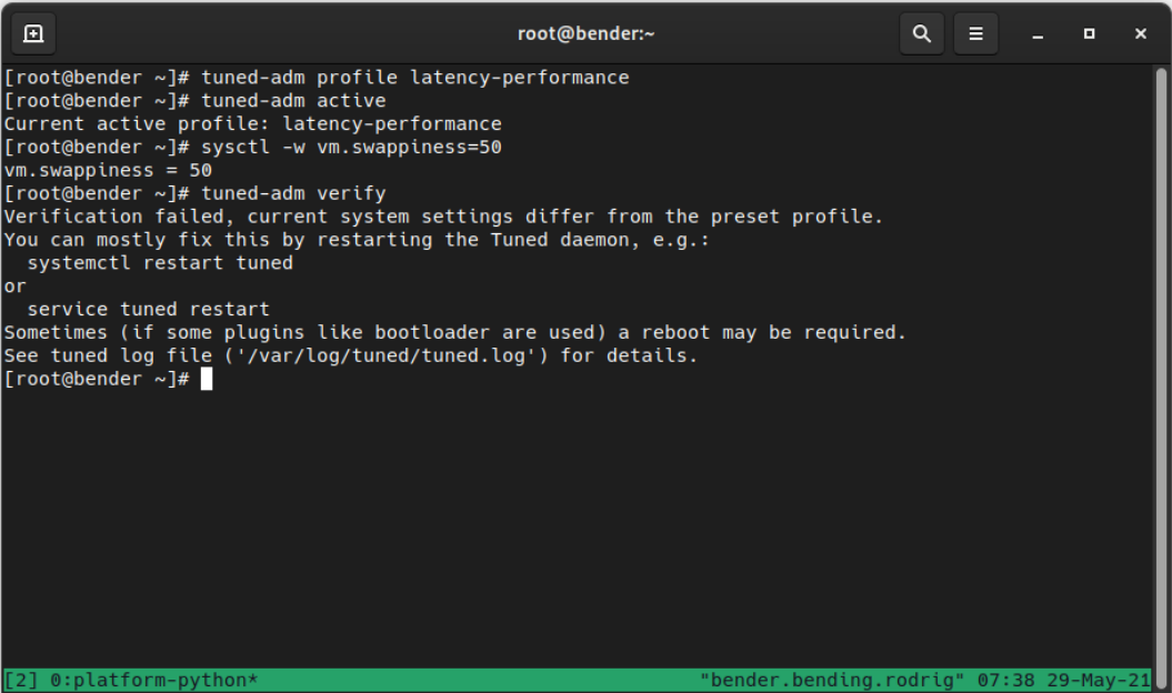
Figure 16.6 – The tuned-adm profile activation and verification
