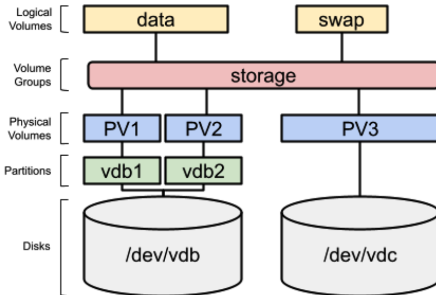
Figure 13.12 – Volume group with logical volume removed
