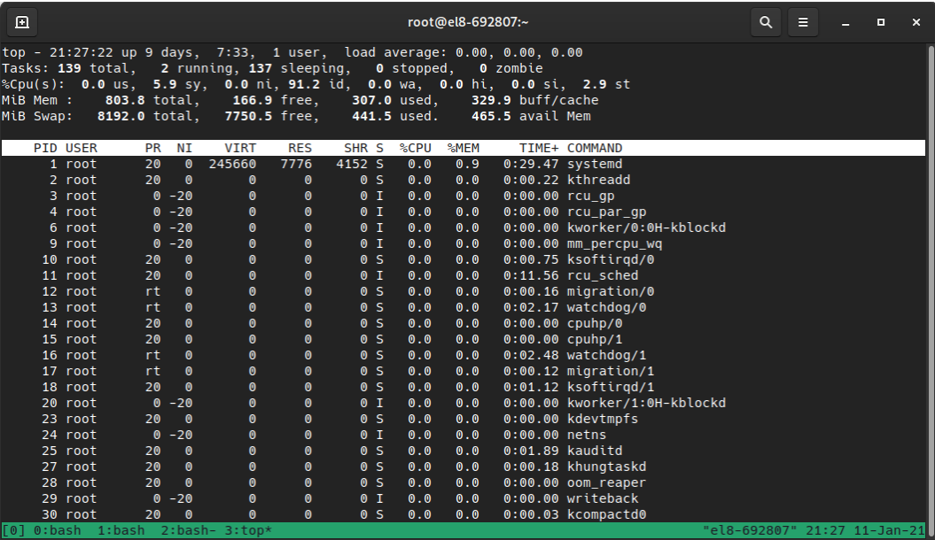
Figure 4.8 – top execution on our test system
