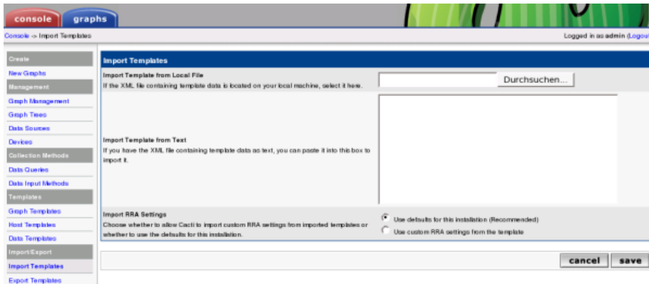
Figure 13-4. Import Templates
