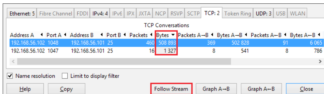
TCP Conversations sorted by Bytes
