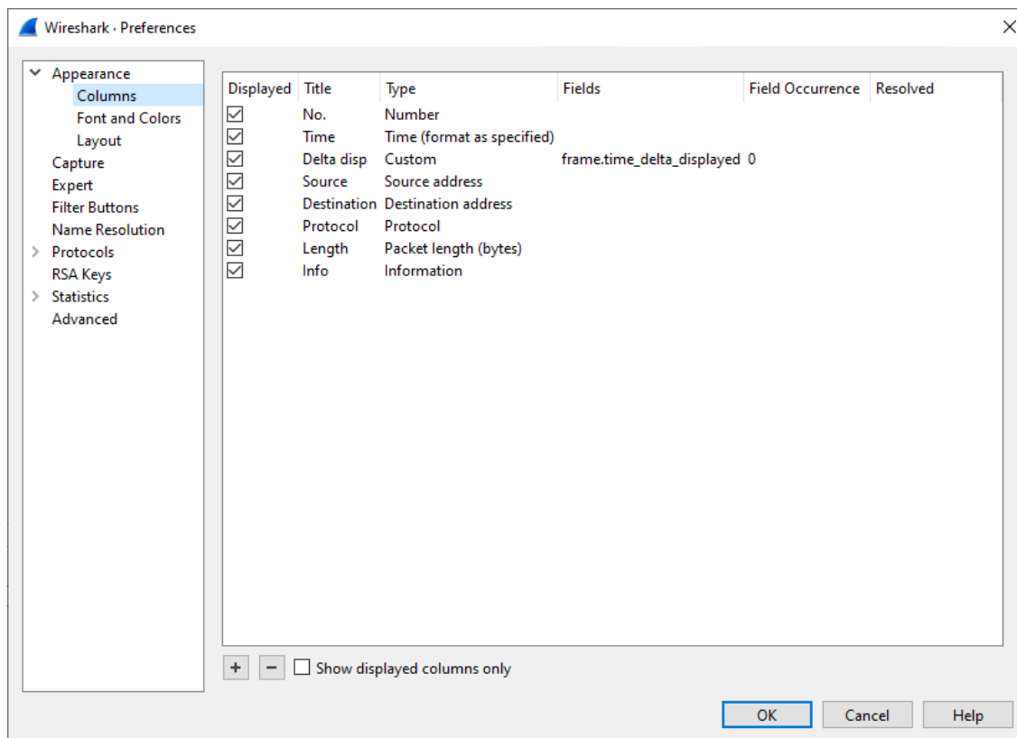
Figure 124. Column preferences
