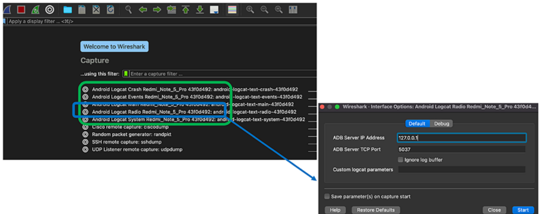
Figure 2-9. Androidddump interfaces
