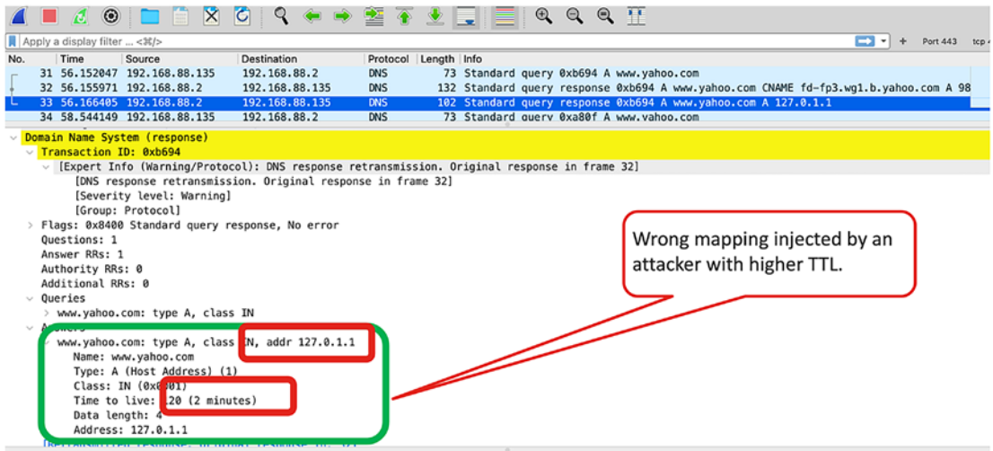
Figure 8-4. DNS spoofing
