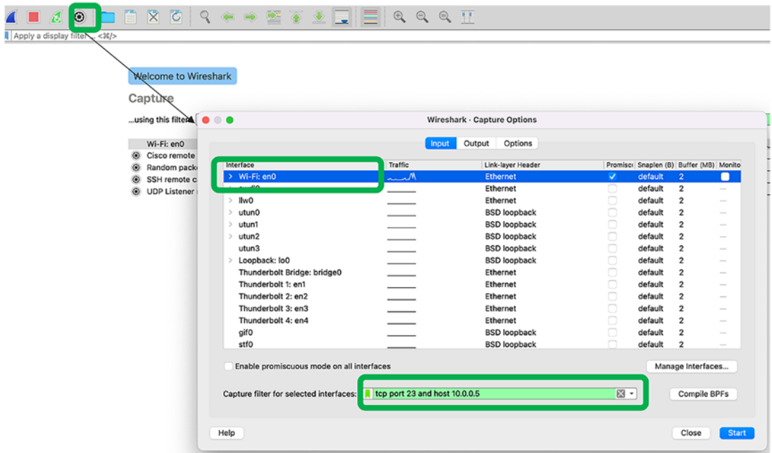
Figure 2-15. Capture filter
