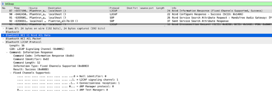
Figure 7-5. L2CAP packet filter
