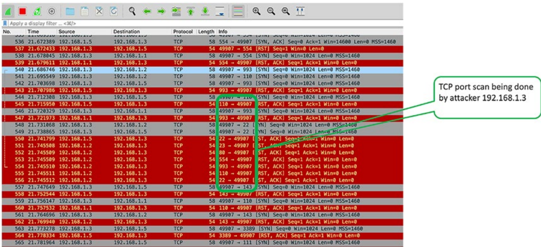
Figure 8-7. TCP port scan
