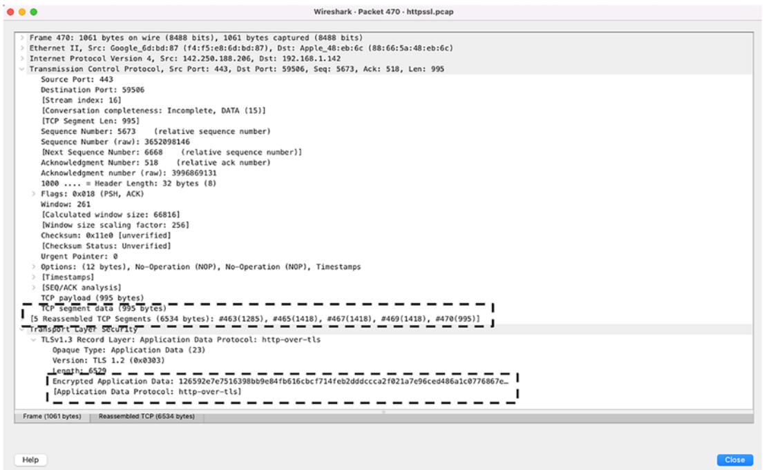
Figure 3-8. Encrypted TLS packet
