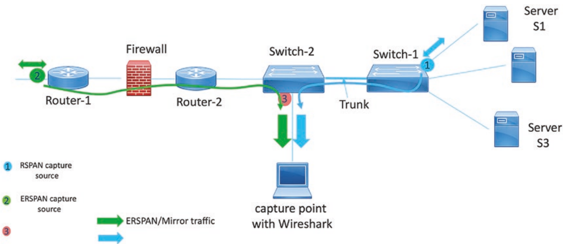
Figure 2-2. Remote port mirroring
