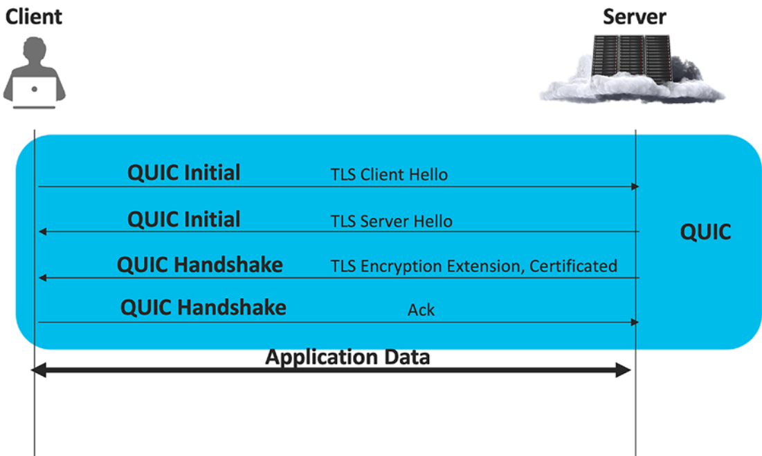
Figure 3-16. QUIC session establishment
