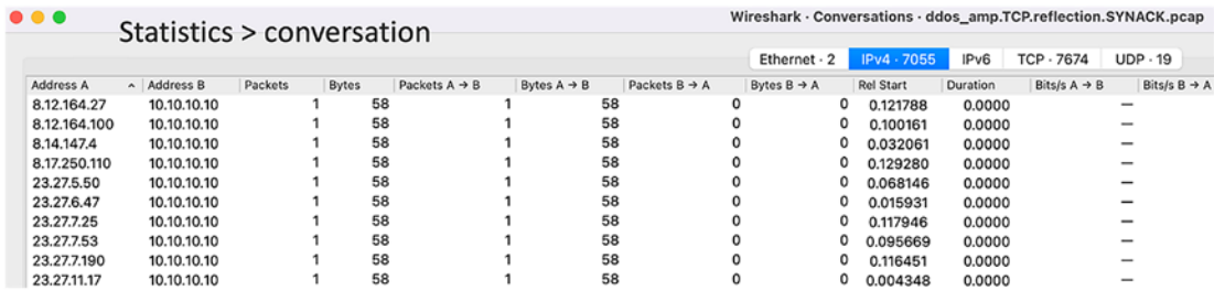
Figure 8-16. Source of the attack
