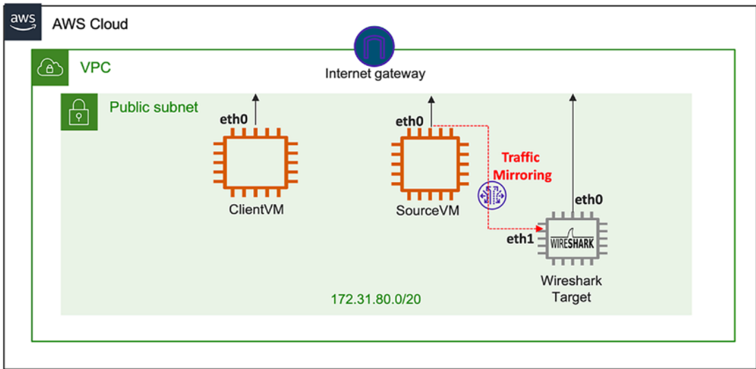
Figure 6-7. AWS VPC example setup
