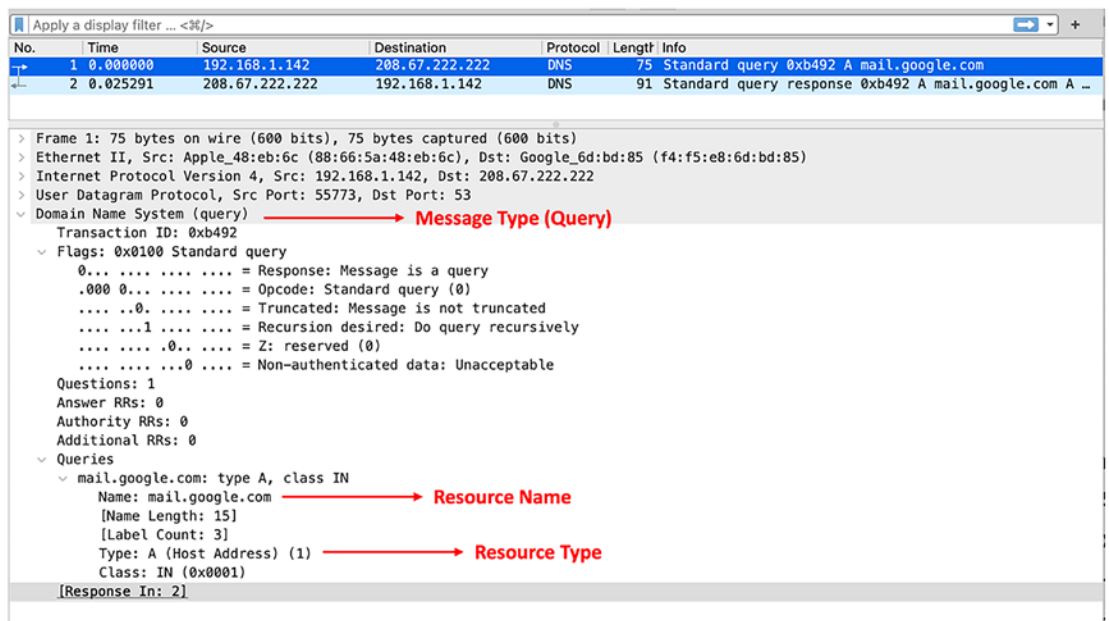
Figure 3-27. DNS Query message
