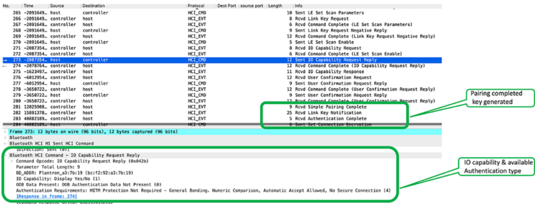
Figure 7-13. Discover I/O capabilities and pair
