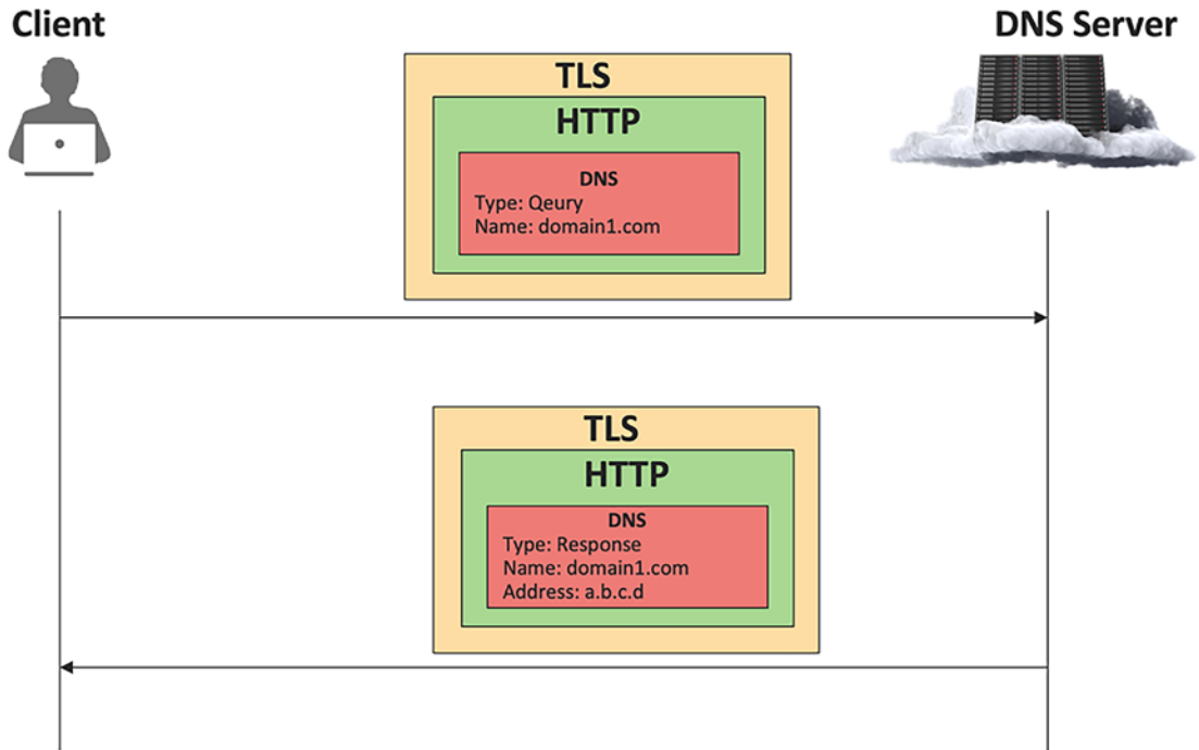
Figure 3-30. Secure domain name resolution
