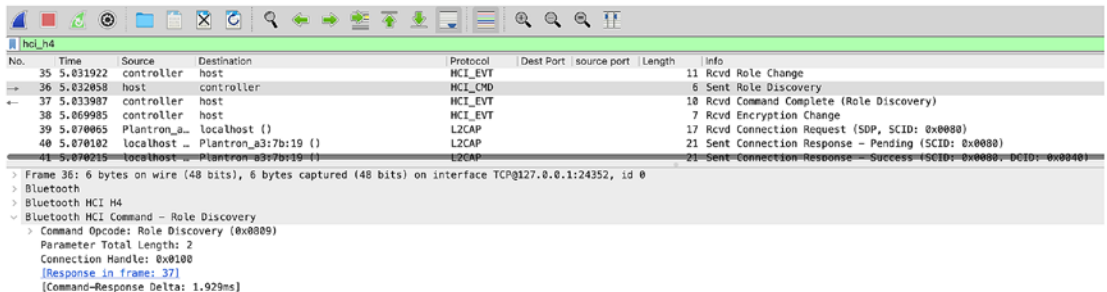
Figure 7-4. HCI packet filter
