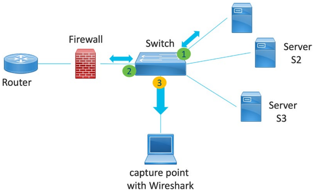
Figure 2-1. Port mirroring
