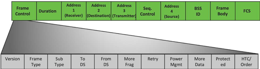
Figure 4-11. IEEE 802.11 frame format
