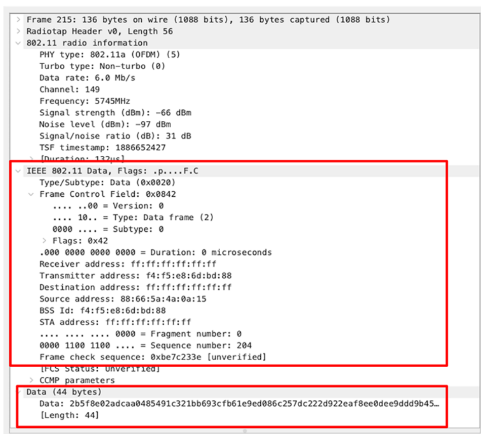
Figure 4-25. 802.11 encrypted data frame
