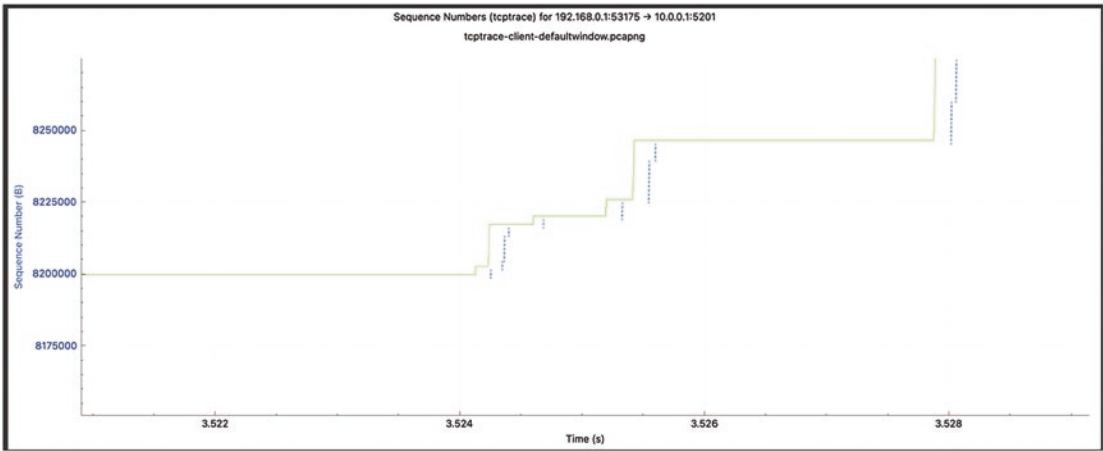
Figure 1-11. TCP stream graphs: time sequence (tcptrace)
