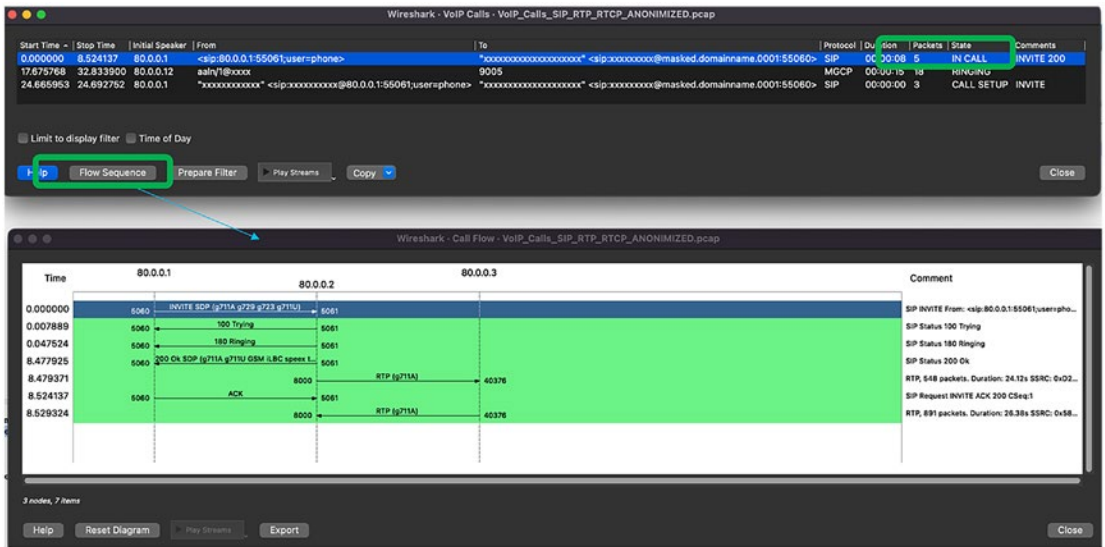
Figure 5-16. VoIP calls and call flow sequence ladder diagram
