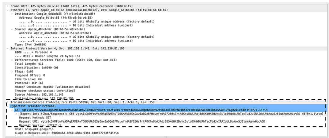
Figure 3-2. Wireshark capture of an HTTP packet
