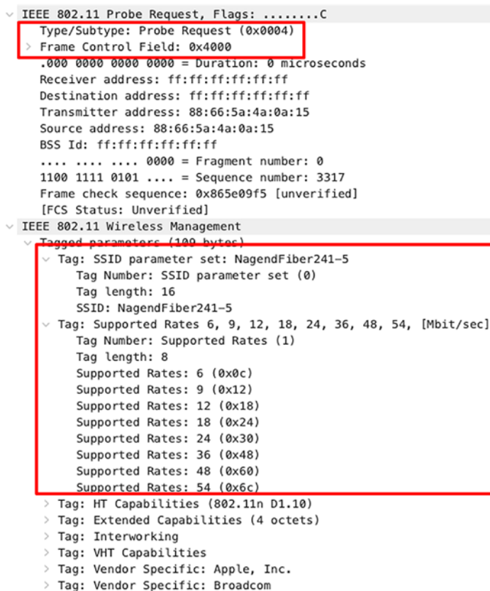
Figure 4-17. Probe Request frame
