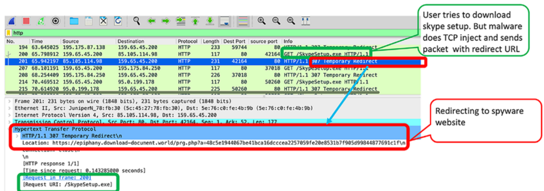
Figure 8-12. Turkish malware redirect
