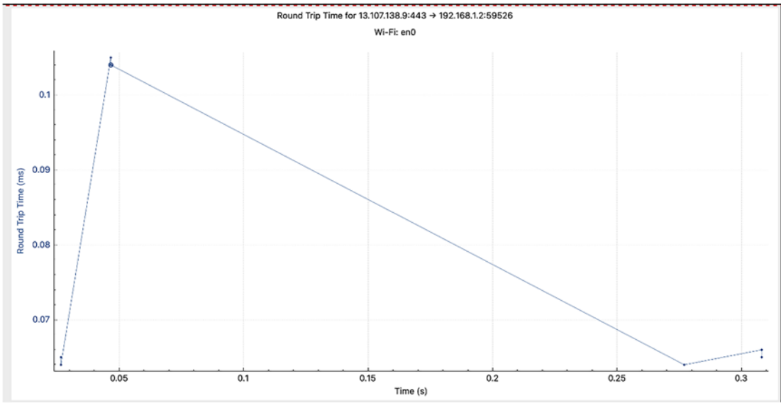
Figure 1-13. TCP stream graphs: round trip time
