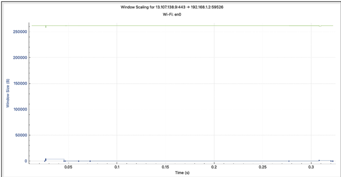
Figure 1-14. TCP stream graphs: window scaling
