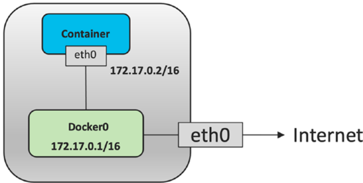
Figure 6-21. Docker default bridge
