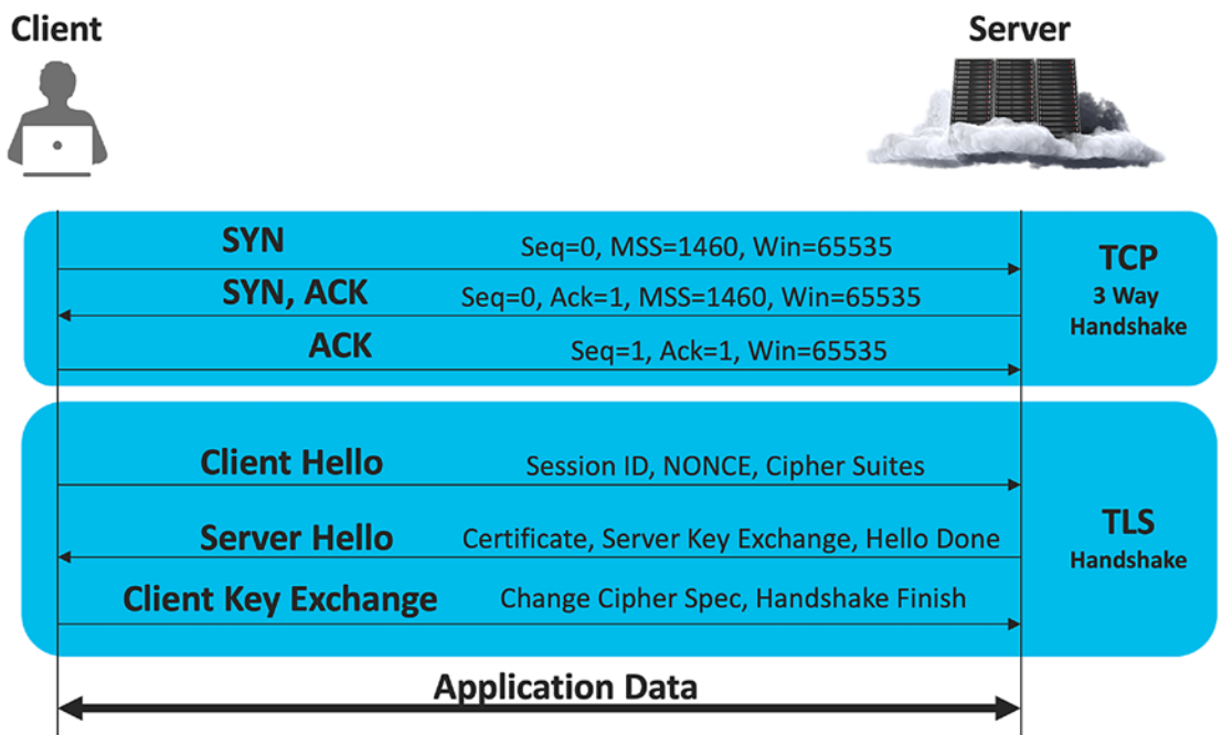
Figure 3-3. TCP+TLS session establishment
