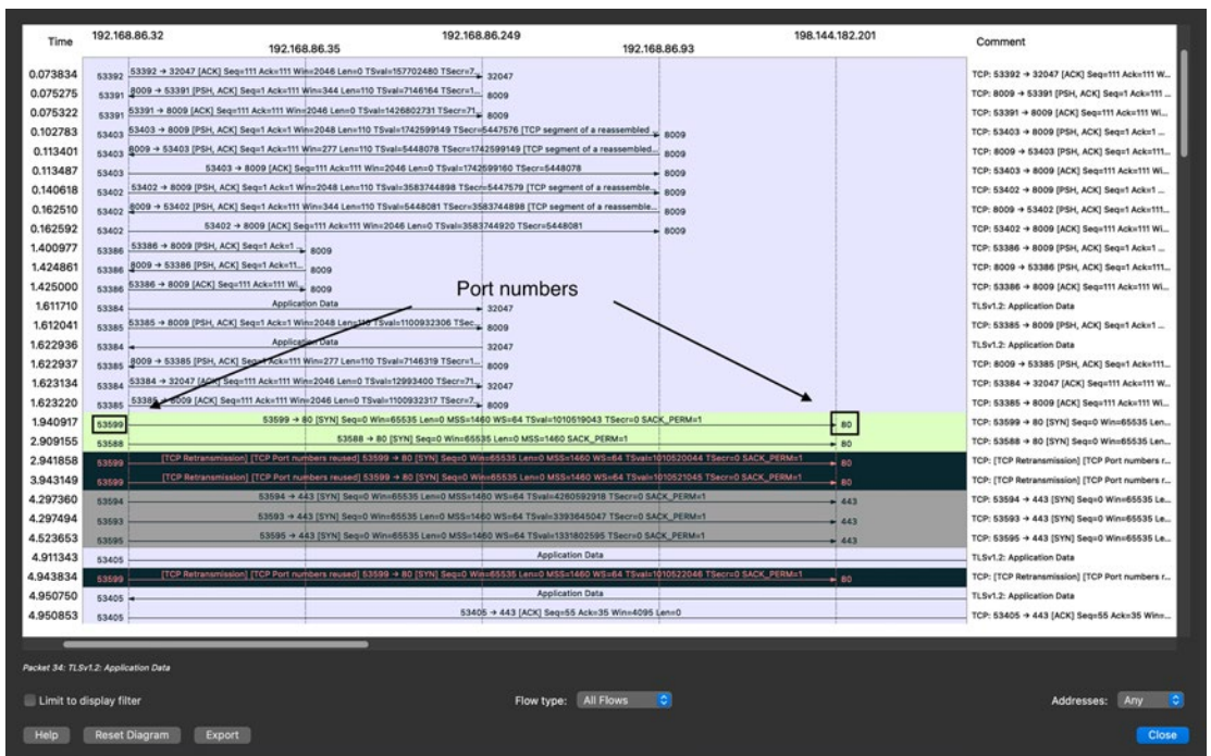
Figure 1-17. Flow graph
