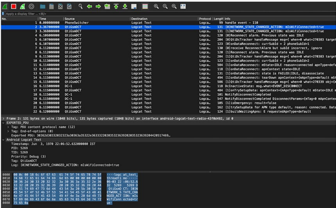
Figure 2-10. Androiddump capture
