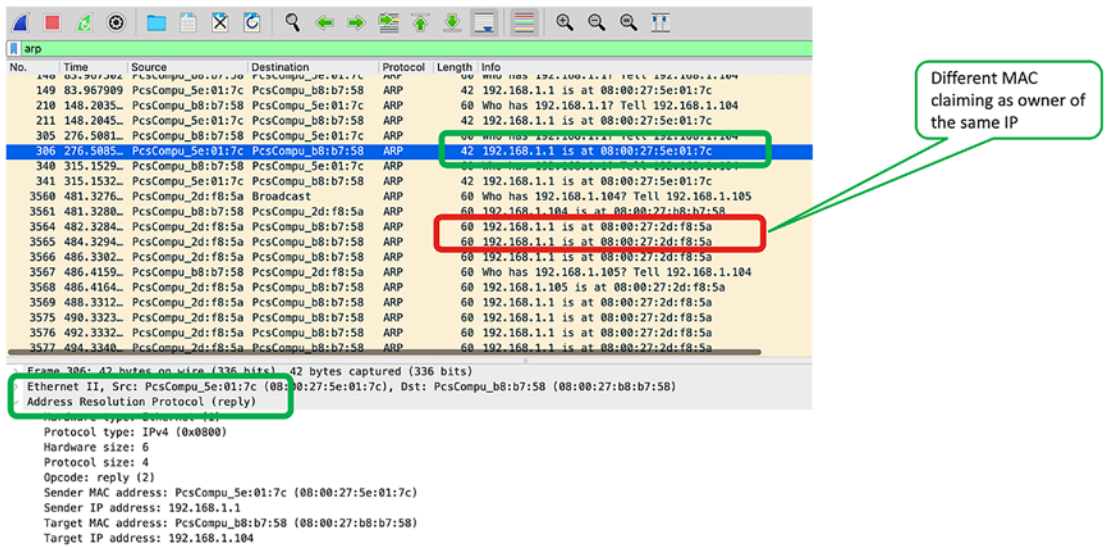
Figure 8-1. ARP spoofing
