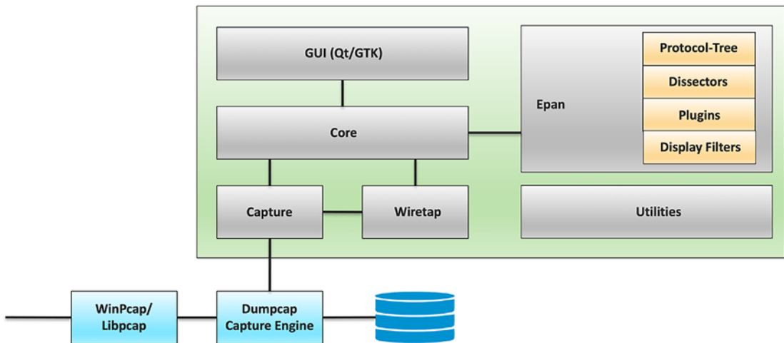
Figure 9-1. Wireshark architecture
