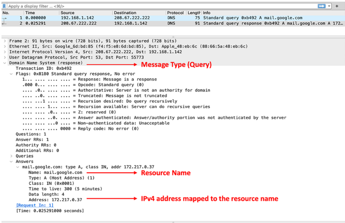
Figure 3-29. DNS response
