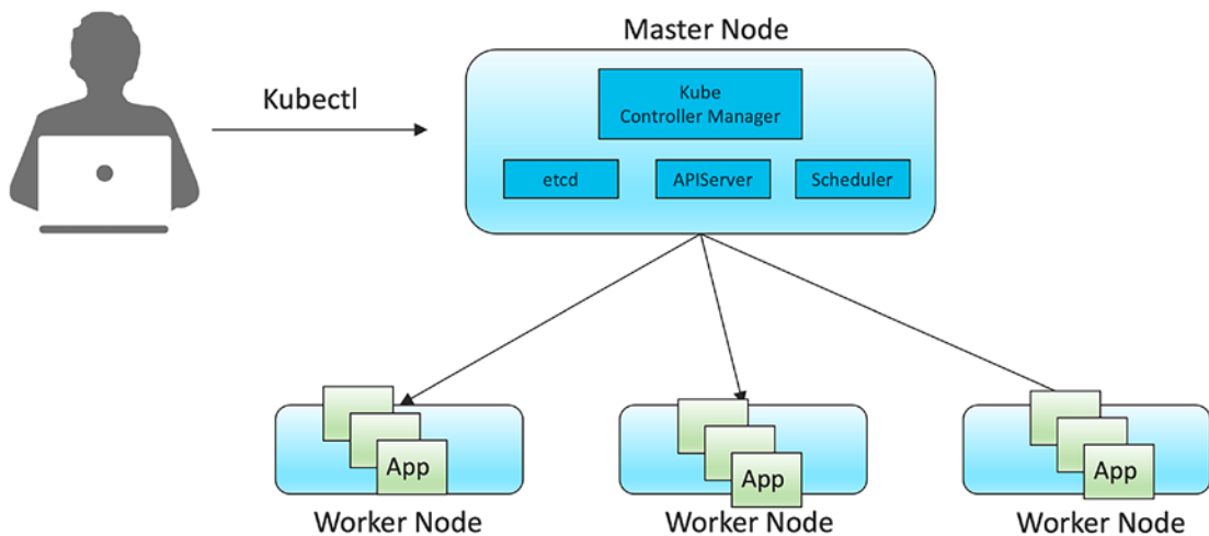
Figure 6-23. Kubernetes architecture
