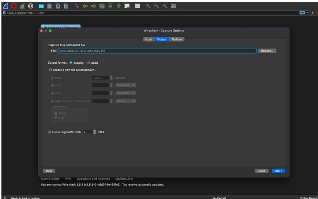
Figure 1-8. Capture options
