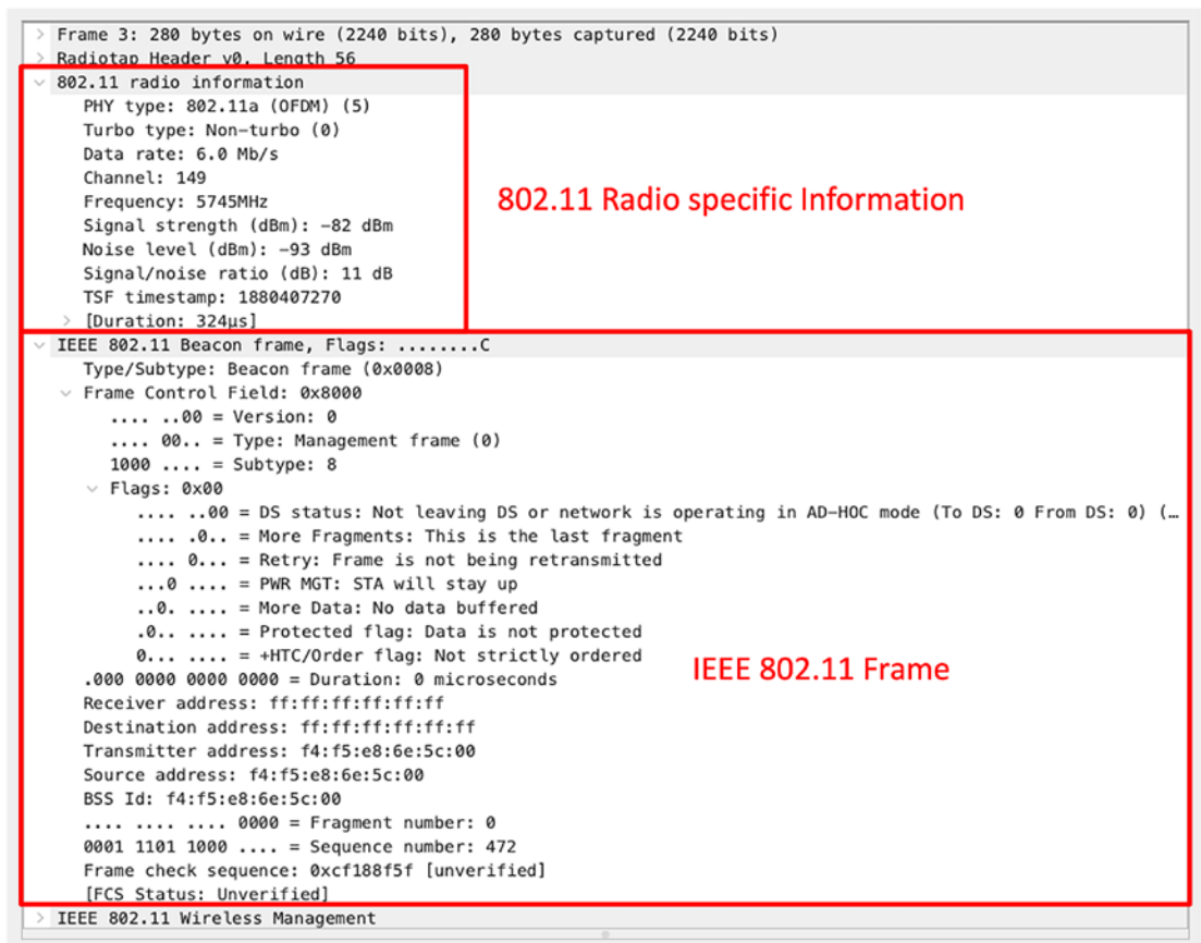
Figure 4-12. 802.11 management frame
