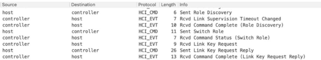
Figure 7-14. Link scan role discovery and key exchange
