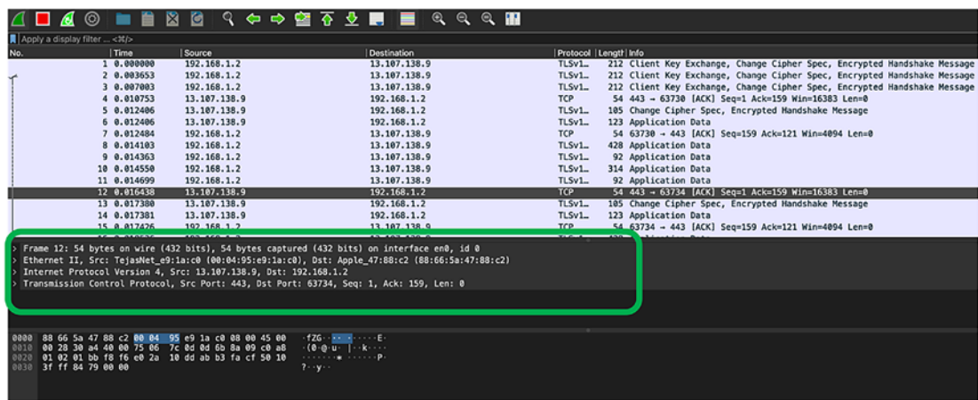
Figure 1-4. Understanding a packet capture
