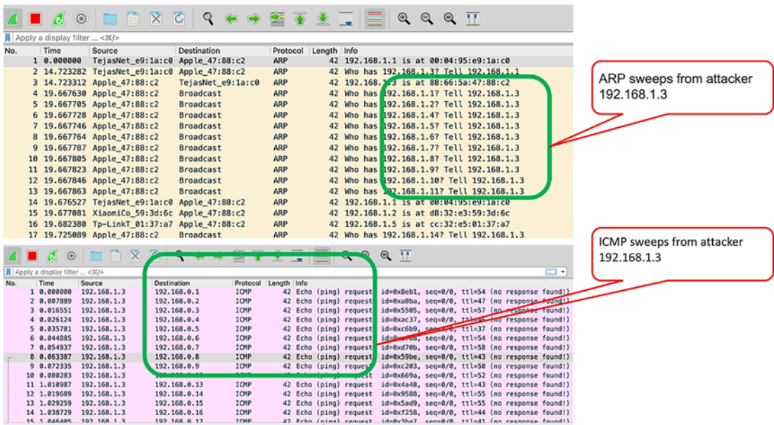
Figure 8-5. Sweep attacks – ARP and ICMP
