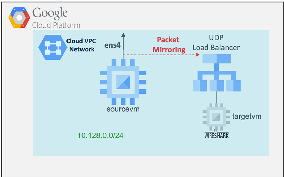
Figure 6-15. GCP VPC example setup
