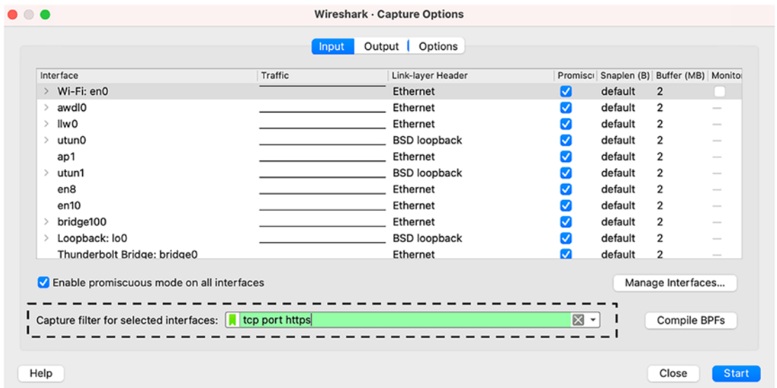
Figure 3-4. Wireshark Capture Options for HTTPS
