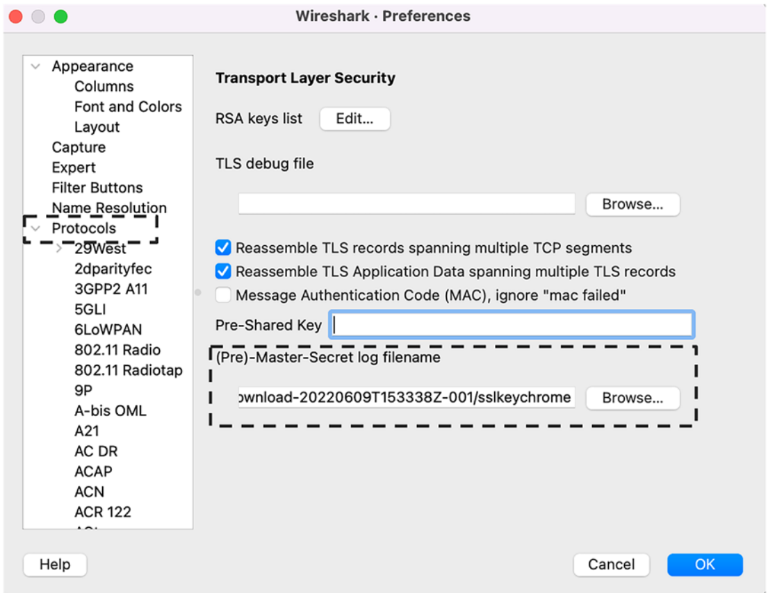
Figure 3-11. Wireshark preference option for the SSL key
