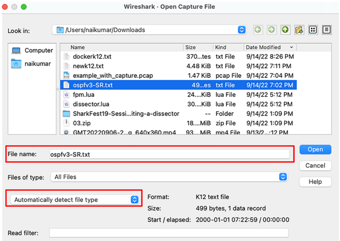
Figure 9-15. Opening text packet file
