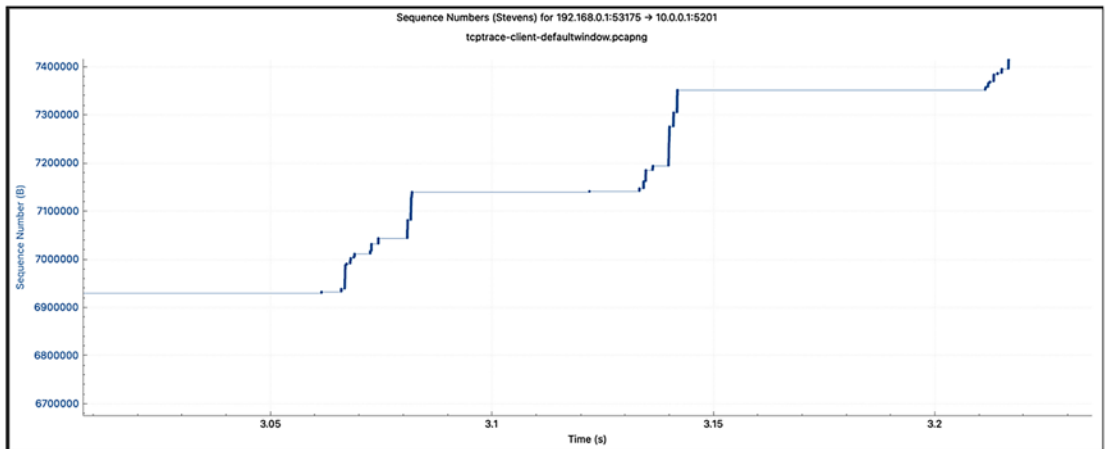
Figure 1-10. TCP stream graphs – time sequence (Stevens)
