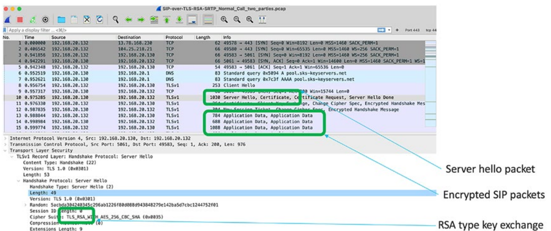
Figure 5-9. SIP over TLS packets - encrypted
