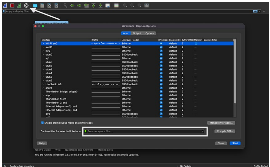
Figure 1-5. Capture filter
