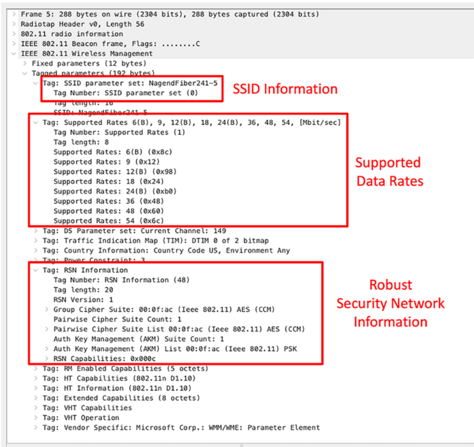
Figure 4-15. 802.11 beacon frame
