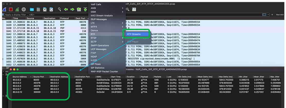
Figure 5-18. RTP streams
