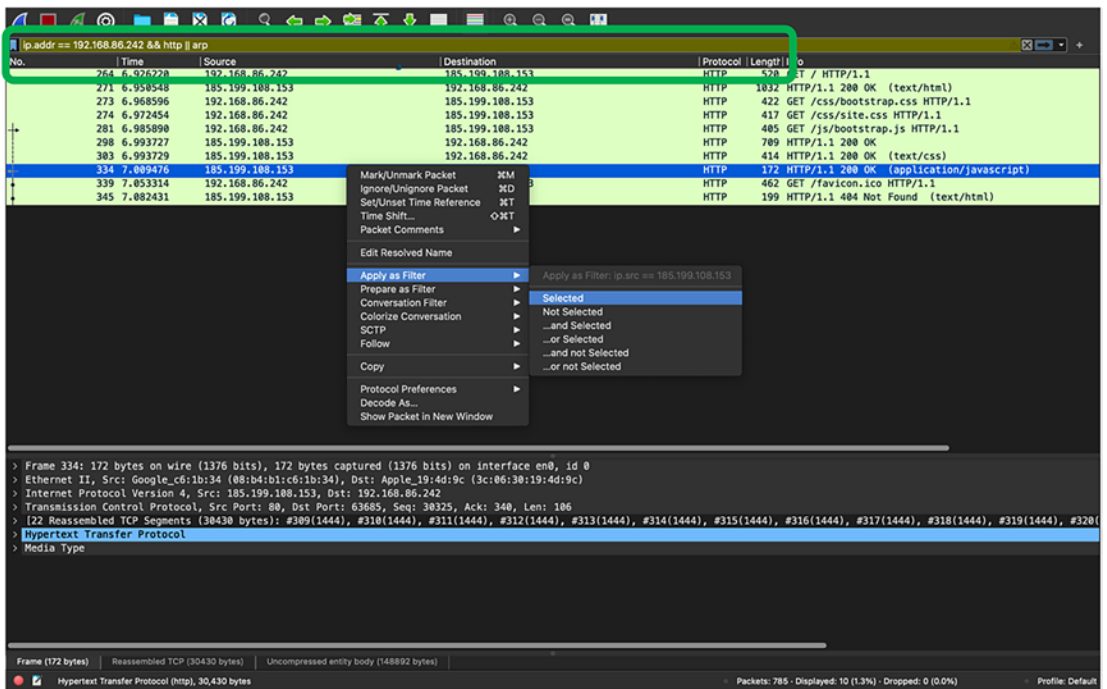
Figure 1-6. Display filter
