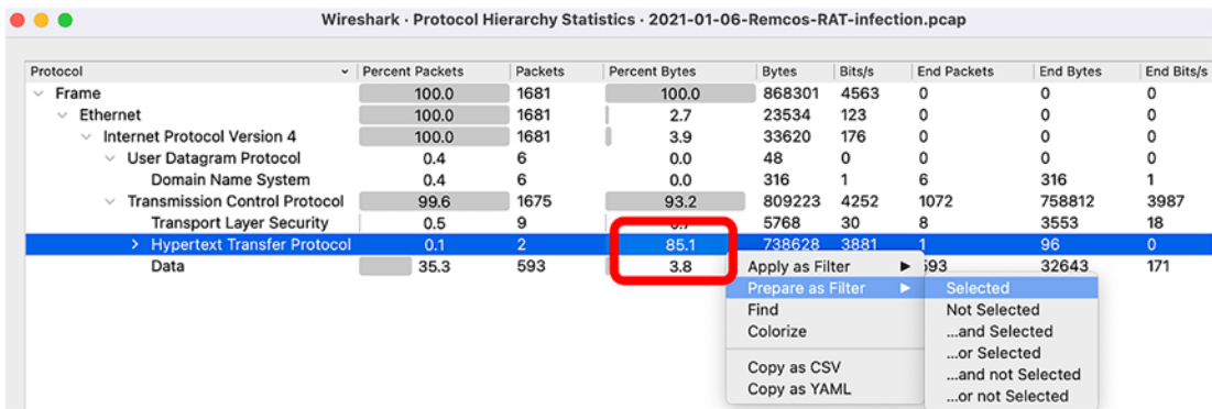
Figure 8-20. Protocol hierarchy
