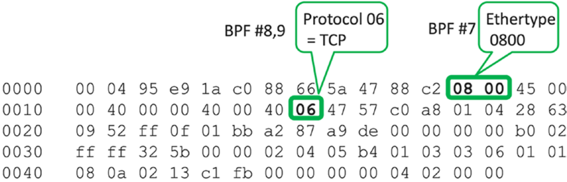
Figure 2-16. BPF example
