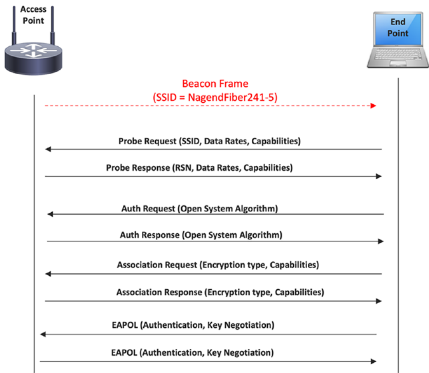
Figure 4-16. Registration process
