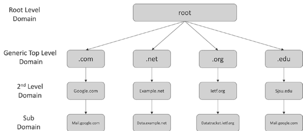
Figure 3-28. DNS hierarchy
