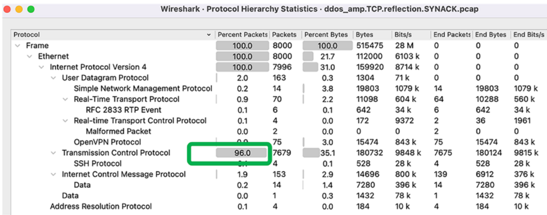
Figure 8-18. Protocol hierarchy
