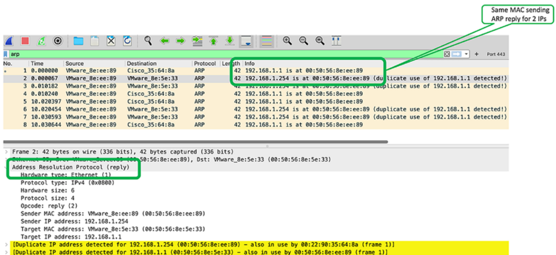
Figure 8-2. ARP poisoning
