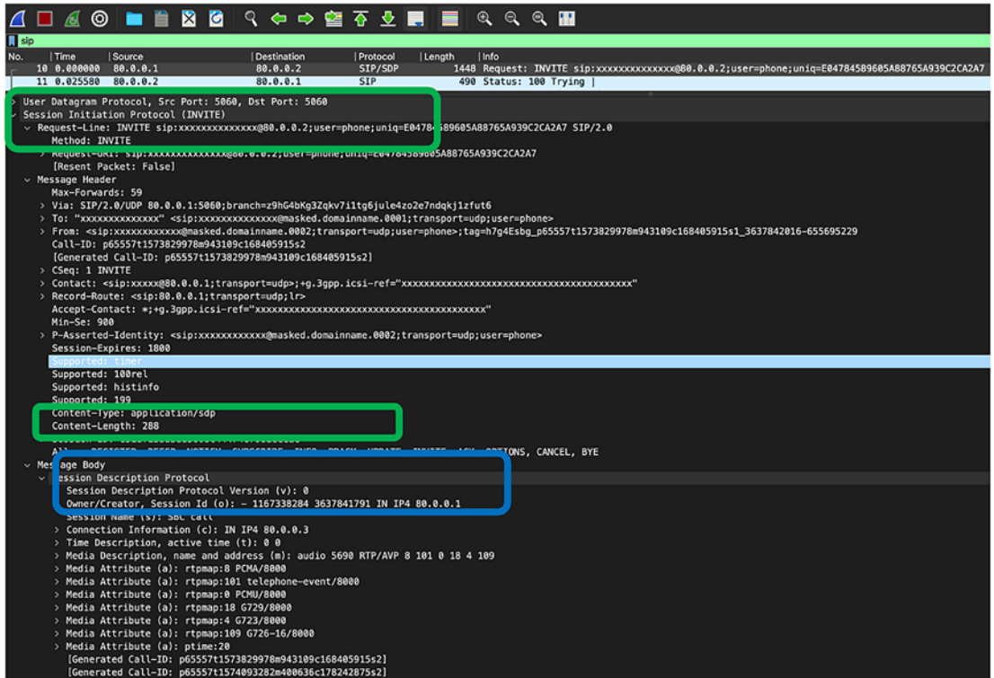
Figure 5-1. SIP and SDP
