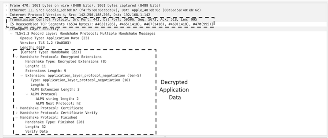
Figure 3-12. Decrypted TLS packet
