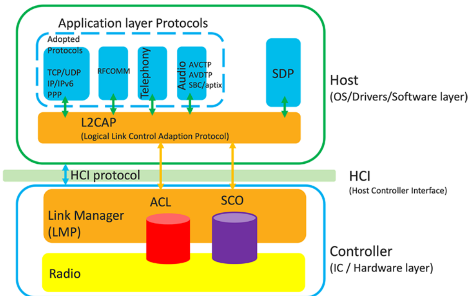
Figure 7-3. Bluetooth protocol stack
