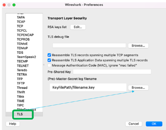
Figure 5-5. Premaster keylog file
