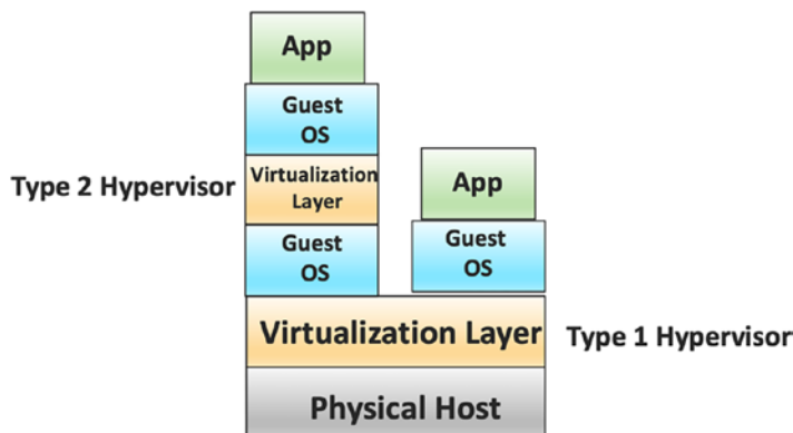
Figure 6-3. Hypervisor types
