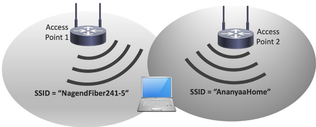
Figure 4-14. 802.11 SSID broadcast
