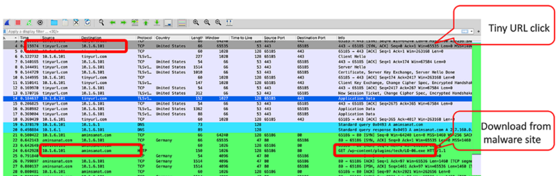
Figure 8-19. Malware download
