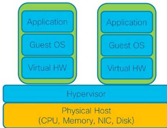
Figure 6-4. Virtual machines
