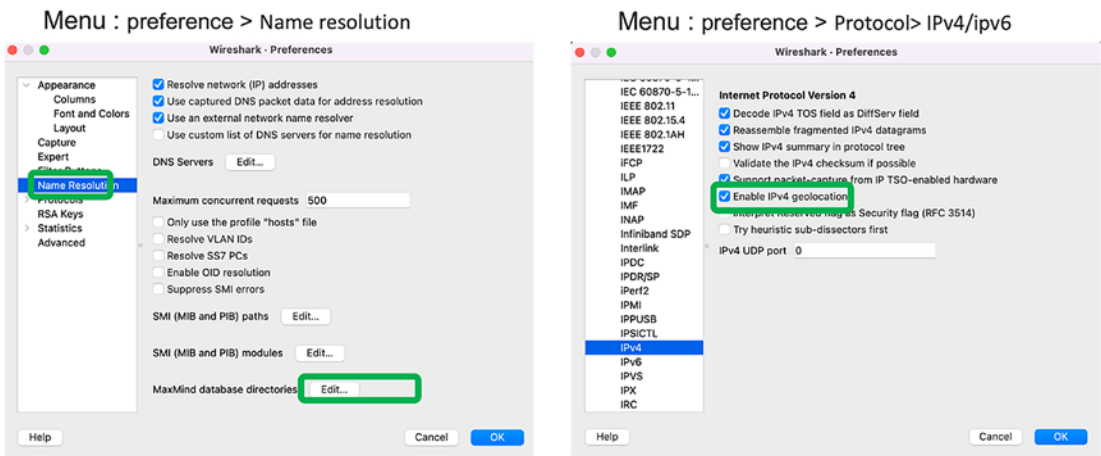
Figure 8-13. Enabling geolocation
