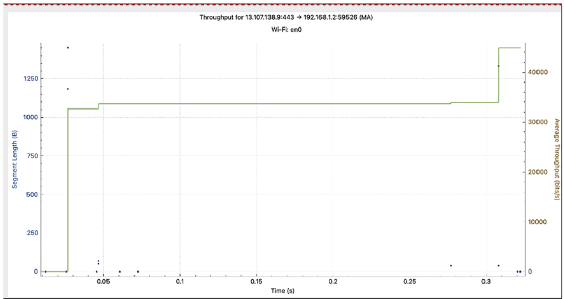
Figure 1-12. TCP stream graphs: throughput
