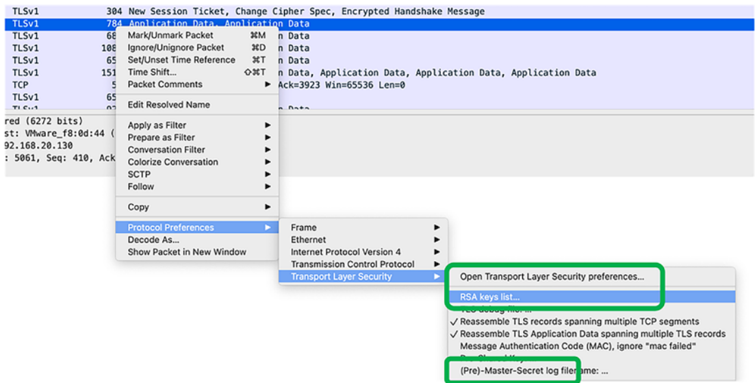
Figure 5-8. TLS packet protocol preference
