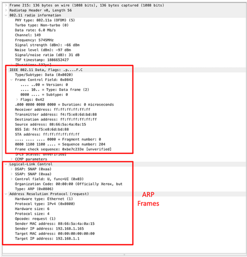
Figure 4-29. 802.11 decrypted data frame
